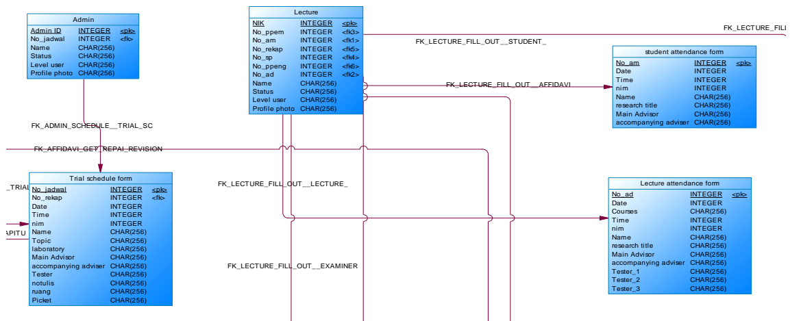
Fig. 9. Physical data model
