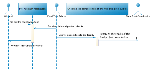
Fig. 5. Prayudisium registration sequence diagram and checking the completeness of prayudisium prerequisites
