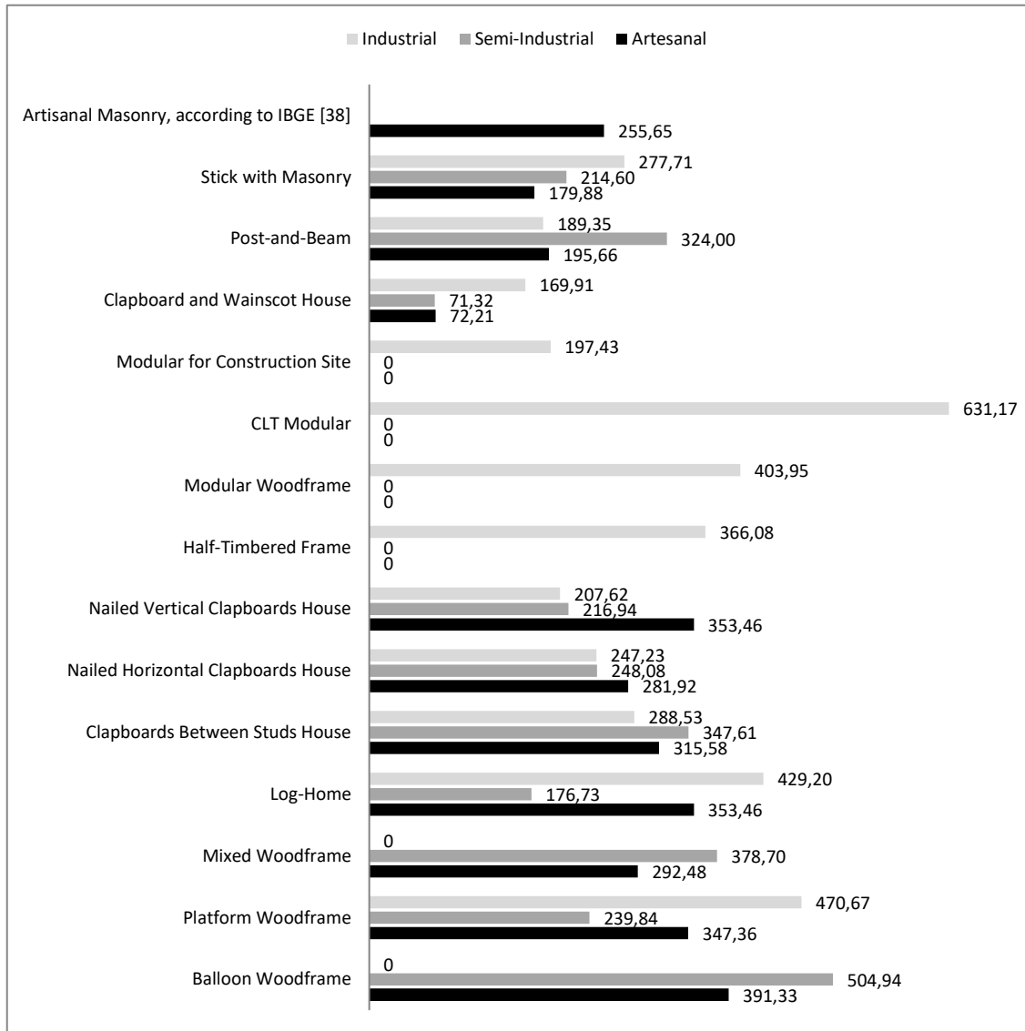
Fig. 2. Basic unitary cost (US$/m 2 ) of timber houses with average finishing standard
