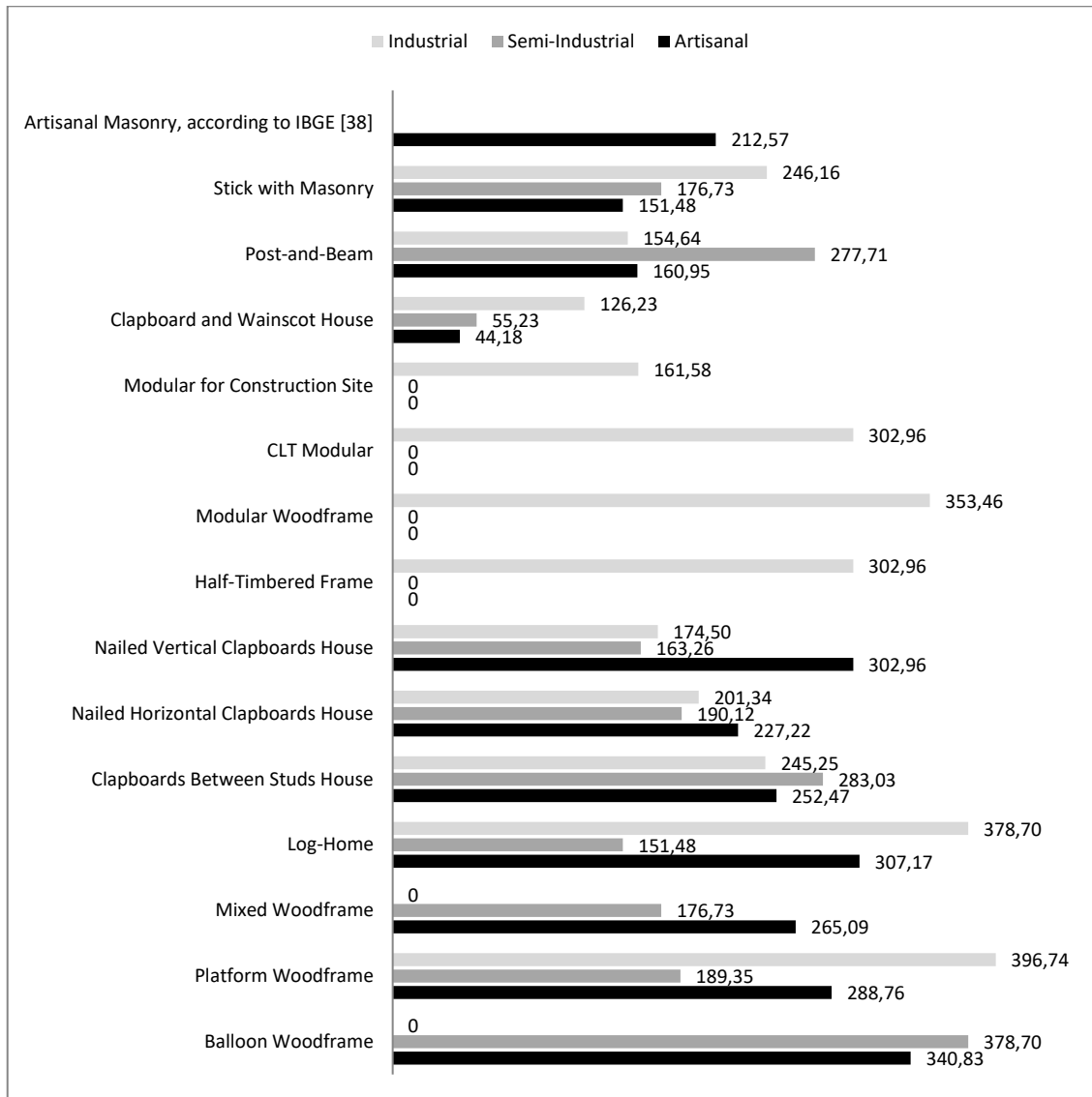
Fig. 1. Basic unitary cost (US$/m 2 ) of timber houses with low finishing standard
