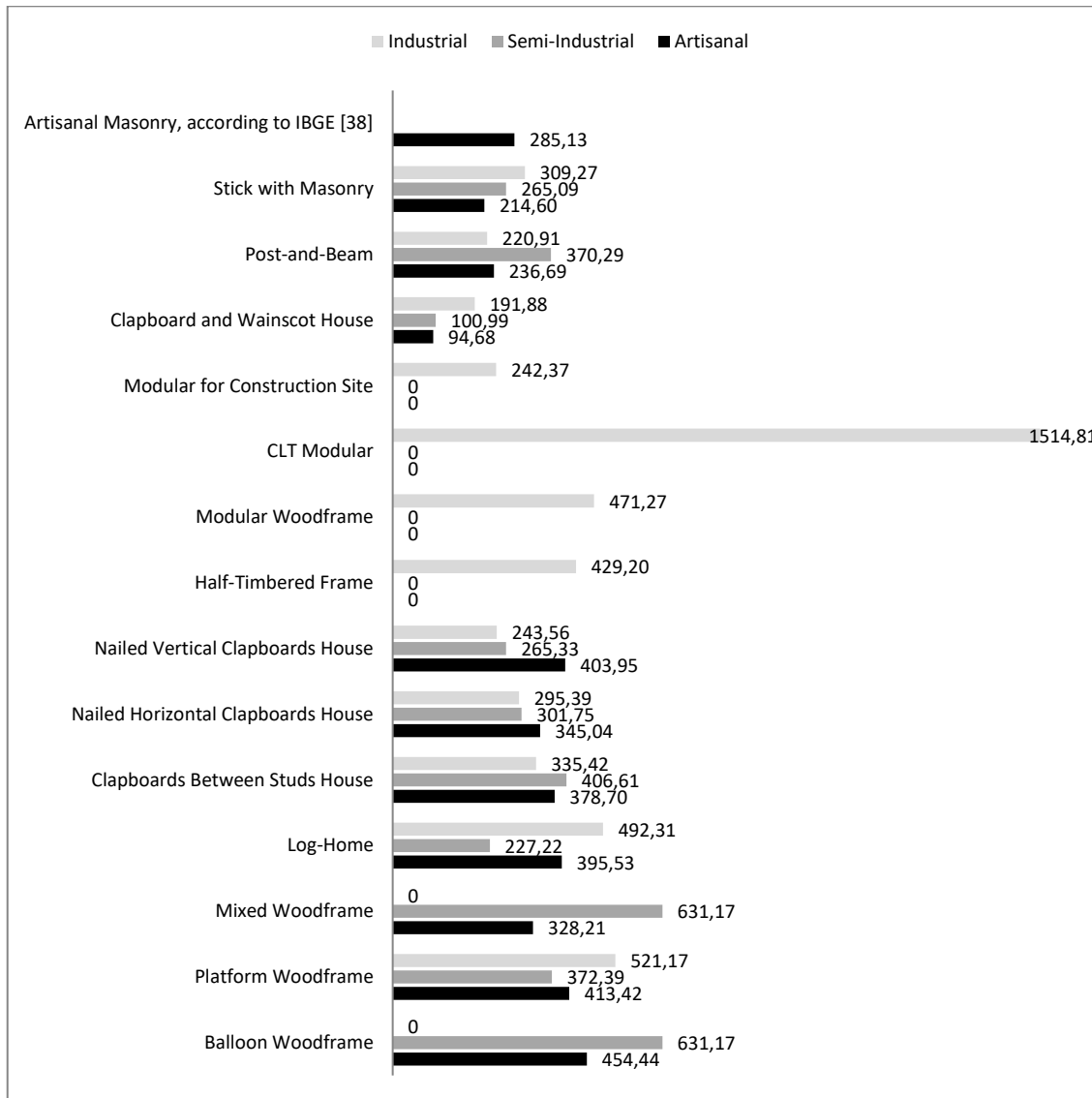
Fig. 3. Basic unitary cost (US$/m 2 ) of timber houses with high finishing standards
