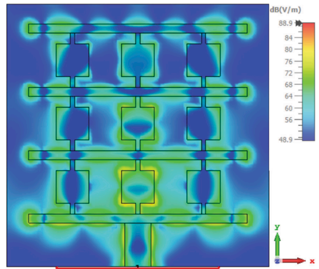
Fig. 4. Surface current density distribution over the proposed array at its resonance frequency of 35 GHz.
