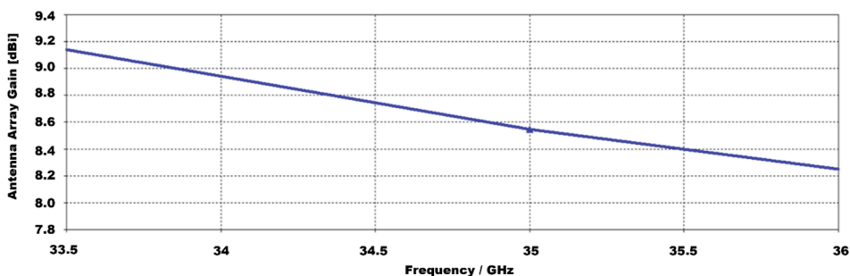
(a) Gain of the proposed basic antenna array
