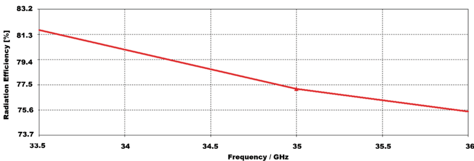
(b) Radiation efficiency of the proposed basic antenna array
