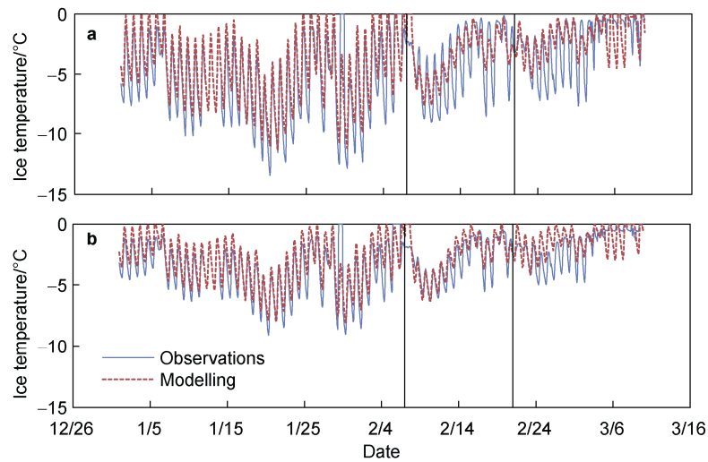
Figure 4 The modelled and measured ice temperature at 10 cm (a) and 20 cm (b) depth in winter 2017. The vertical black lines denotes the date of two snowfall events.
