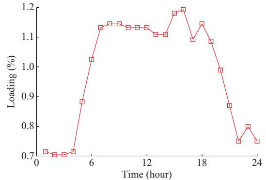
Fig. 4. 24-hour loading profile of network.
