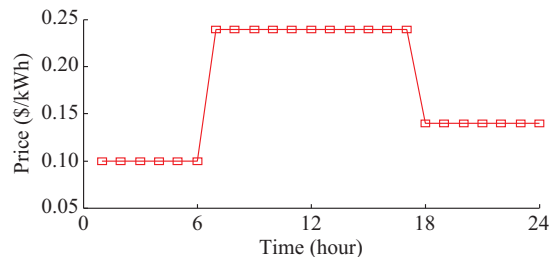
Fig. 5. 24-hour three-level electricity price in power grid.
