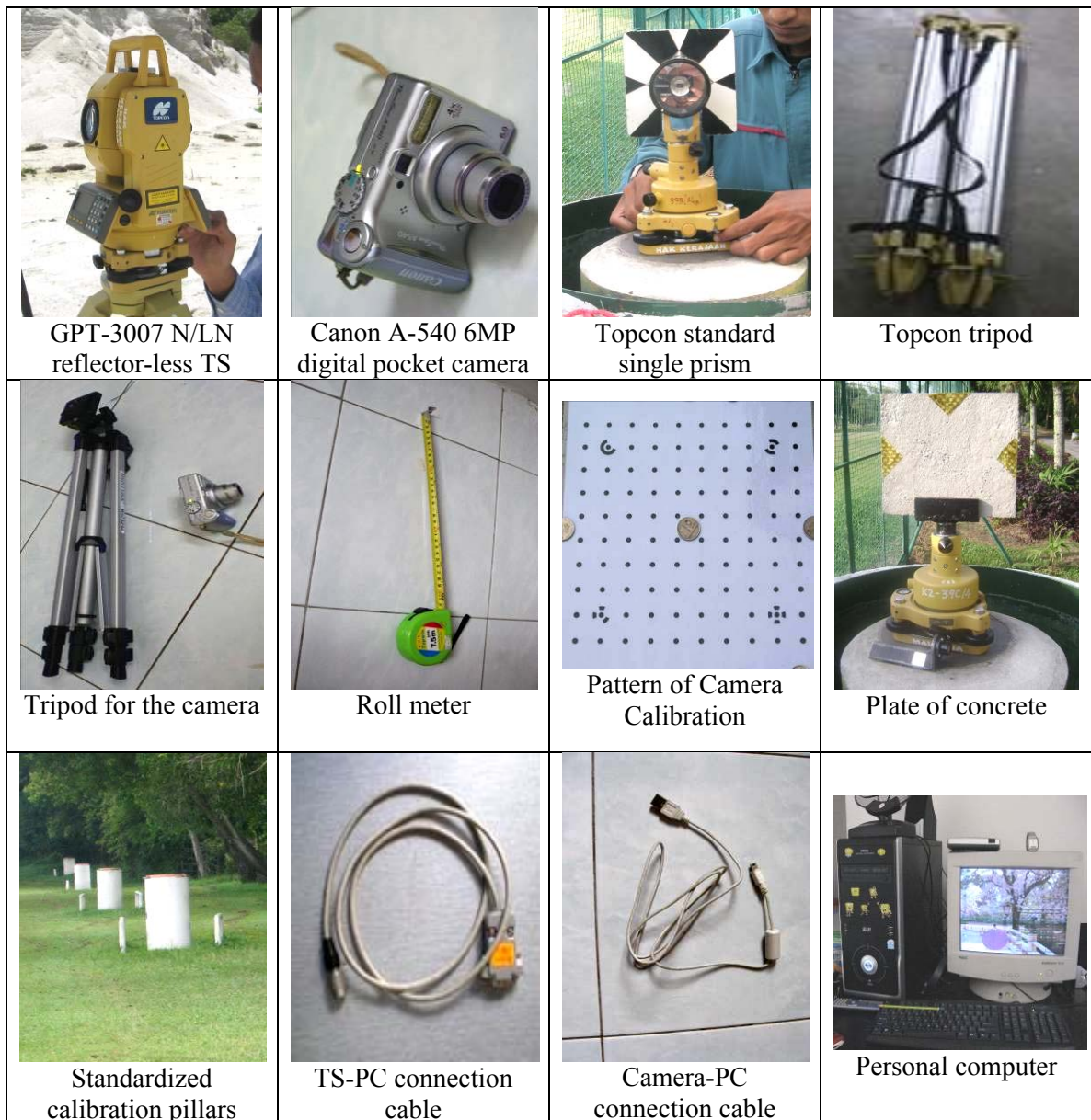
Figure 3.6. Instruments used in this research
