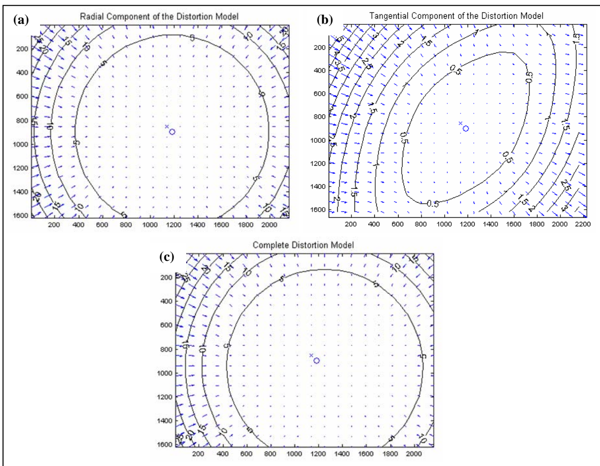
Figure 4.1. Modeling of magnitude and direction for: radial distortion (a); tangential distortion (b); and total lens distortion (c) for Canon A450 with focal length was set on 9.768 mm.
