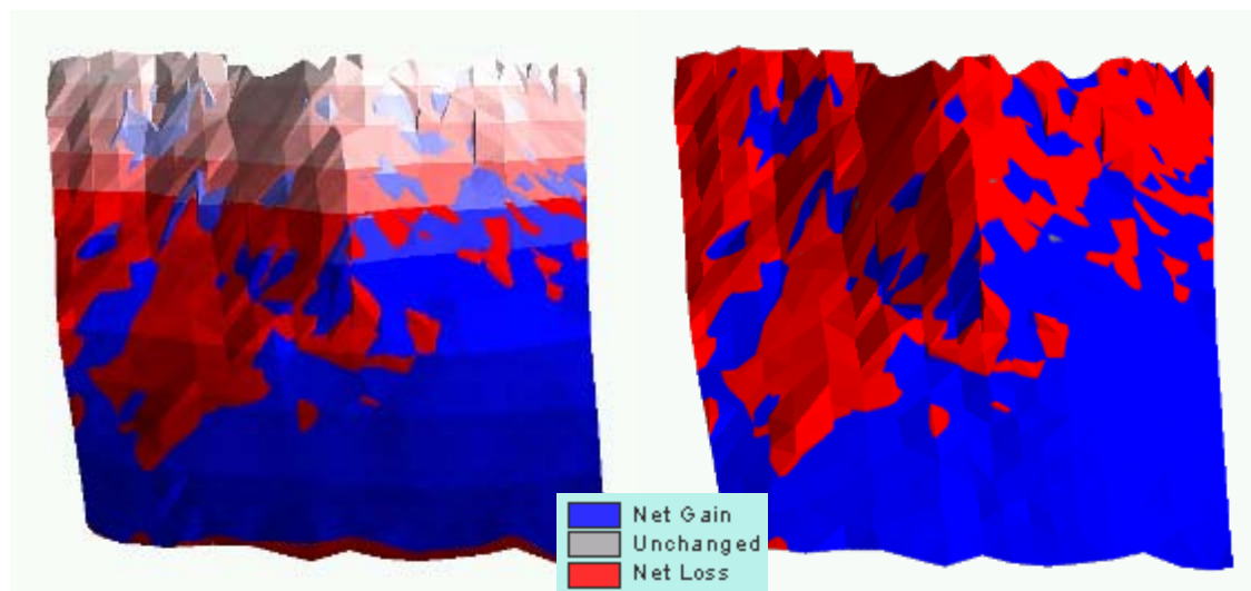
Figure 4.13. The left picture presents overlaying between DEMs of epoch 1 (red graduation) and epoch 2 (blue graduation). Right picture presents the distribution of loss and gain of soil on the slope.
