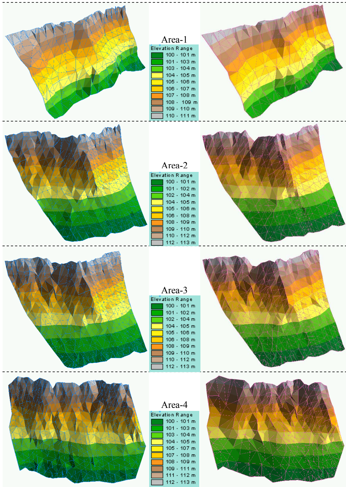
Figure 4.9. Derived DEM generated from total station data (right); and close-range photogrammetric data (left) selected by regular sampling method.
