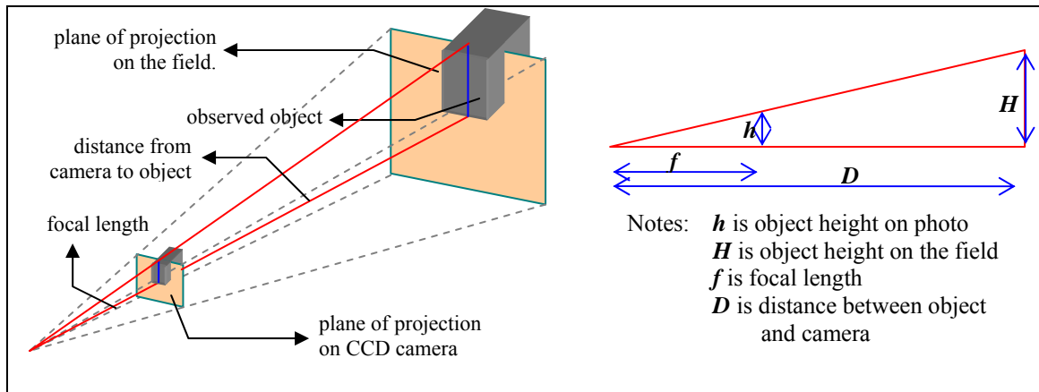
Figure 3.10. Scaling factor calculation illustrated in 3D (left), and in 2D projection by following simple triangles formula (right)
