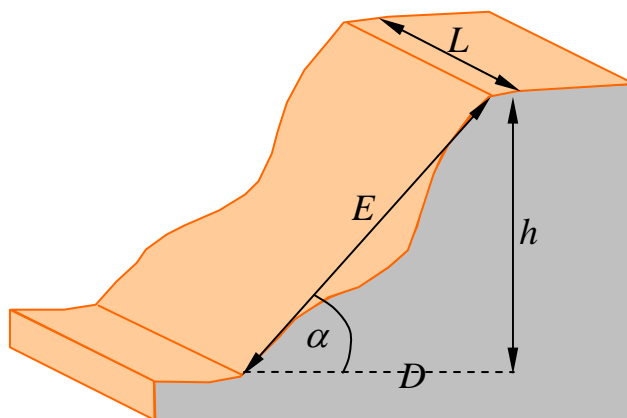
Figure 2.1. Illustration of slope surface (source: [7])
