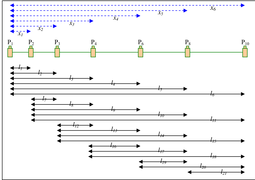
Figure 3.8. Sketch of the pillars (middle picture), with its scenario of the data measurement for all observed sub-baselines (top), and all observed distances (bottom).
