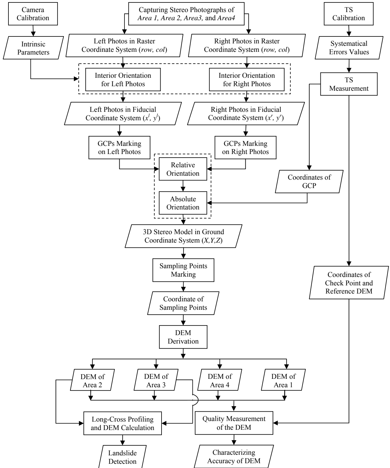
Figure 3.12. Experimental work flow of this research
