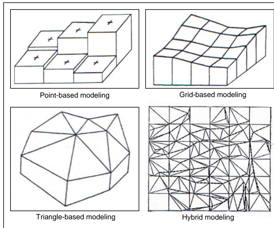
Figure 2.8. Illustration of Digital Elevation Modeling approaches (source: [16])
