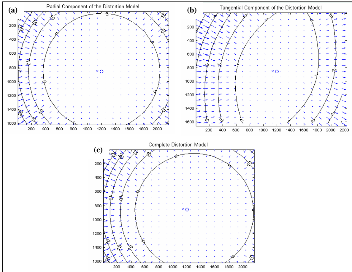
Figure 4.2. Modeling of magnitude and direction for: radial distortion (a); tangential distortion (b); and total lens distortion (c) for Canon A450 with focal length was set on 11.490 mm.
