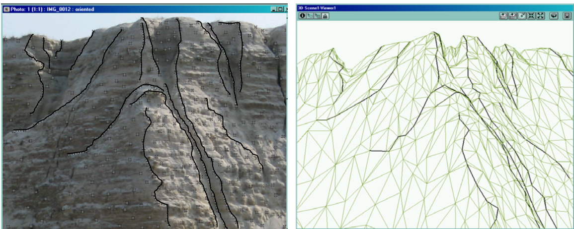
Figure 4.11. Some of digitizing breaklines on the stereo photograph (left); Constructed TIN based on 3D coordinates and breaklines data (right).
