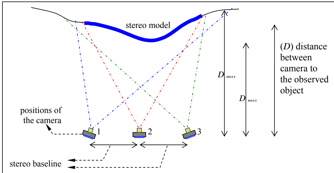
Figure 3.9. Illustration of stereo images data collection
