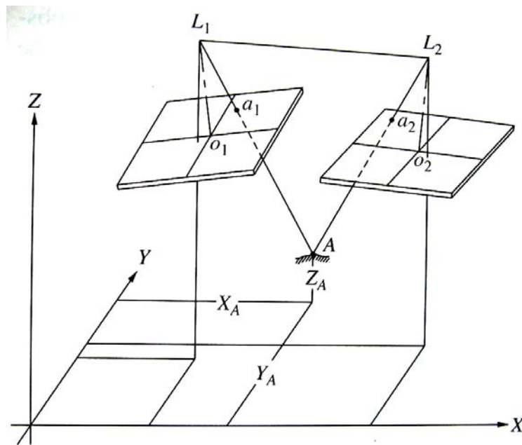
Figure 2.4. Space intersection with a stereo-pair images (source: [3])
