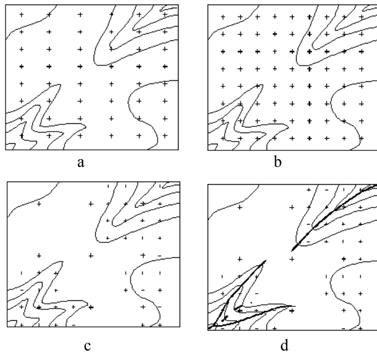
Figure 2.7. Terrain data sampling techniques by using: regular sampling profiling (a), regular grid sampling (b), progressive sampling (c), and selective sampling (d)
