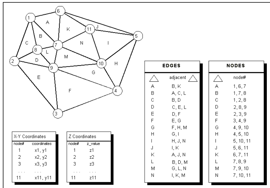
Figure 2.9. Structure of a Triangular Irregular Network (source: [27])
