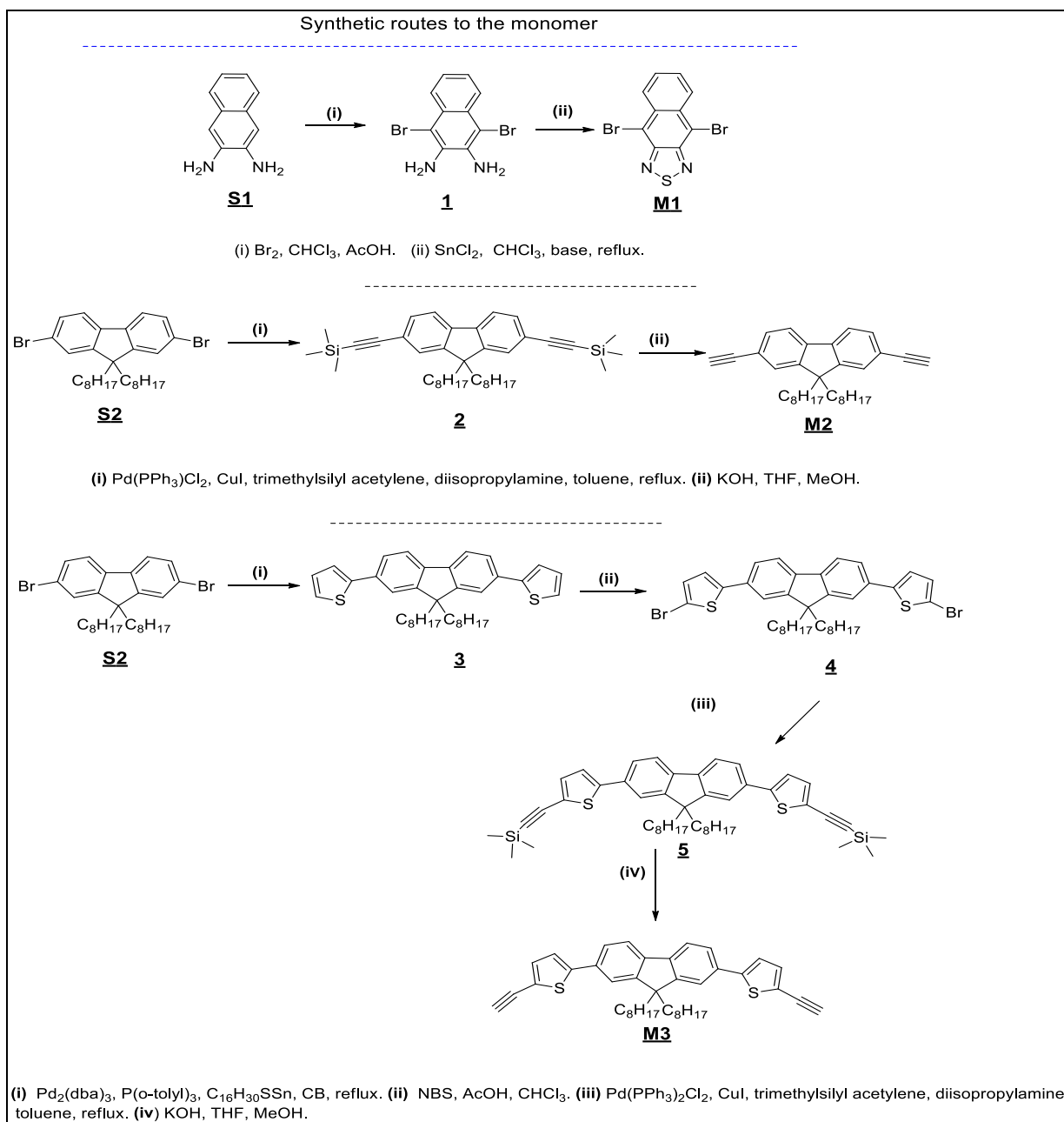
Scheme 1. Synthetic route towards monomers ( M1–M3 ).
