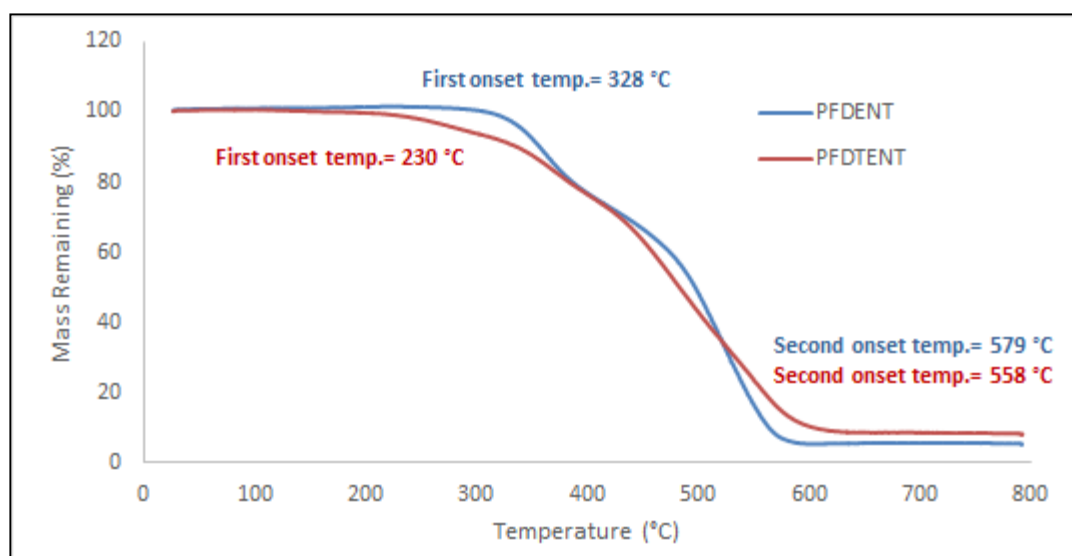
Figure 4. TGA plots of the resulting polymers with a heating rate of 10 °C/min under N 2 .
