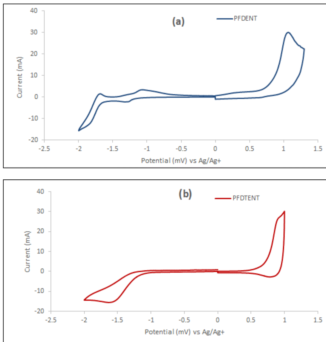
Figure 3. Cyclic voltammograms of (a) PFDENT and (b) PFDTENT.
