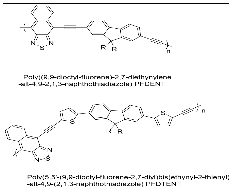
Figure 1. Structures of PFDENT and PFDTENT.
