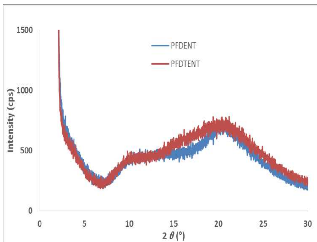
Figure 5. Powder XRD profiles of the target polymers.
