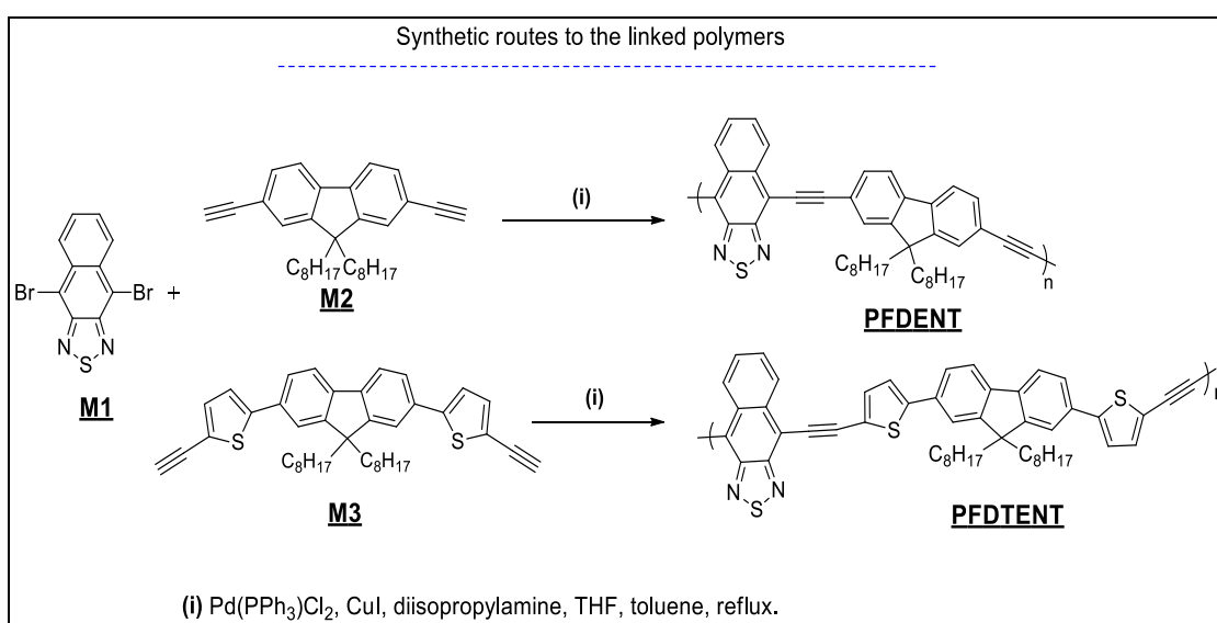
Scheme 2. The synthetic route to polymers and their conditions and reagents.
