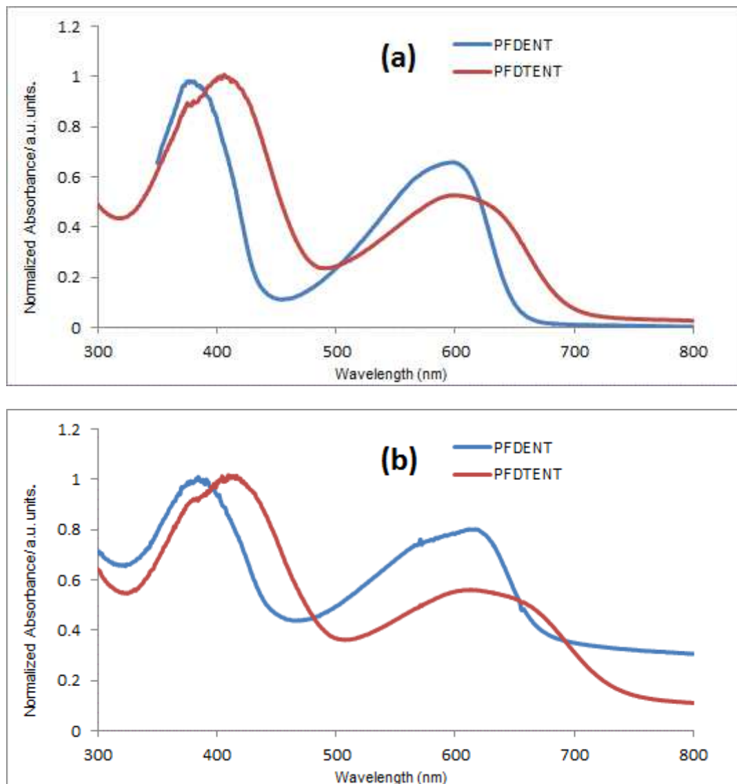
Figure 2. (a) Normalized absorption spectra of polymers in chloroform solution, (b) Absorption spectra of polymers as thin films.
