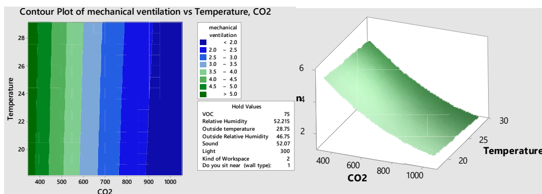
Figure 12. Relationship between temperature and carbon dioxide on indoor air comfort.
