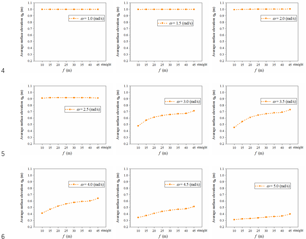
4 5 6 7 Figure 4 Trends of average elevation \eta_a in protection zone, with respect to seven parabolic arc breakwaters with 8 f=10, 15, 20, 25, 30, 35, 40 m and a straight breakwater. w=1 m. d=1 m. \omega=1 to 5 rad/s with an increment of 0.5 9 rad/s.
