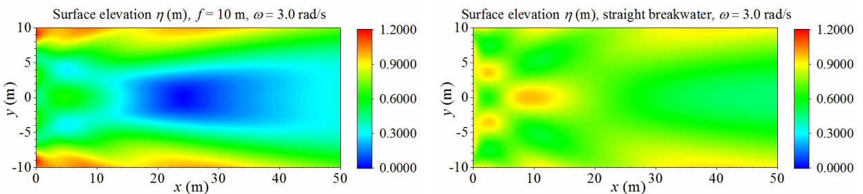
10 11 Figure 5 Surface elevation \eta in the protection zone of the f=10 m parabolic arc breakwater (left) and straight 12 breakwaters (right), where w=1 m, d=1 m, l=20 m, \omega=3 rad/s.
