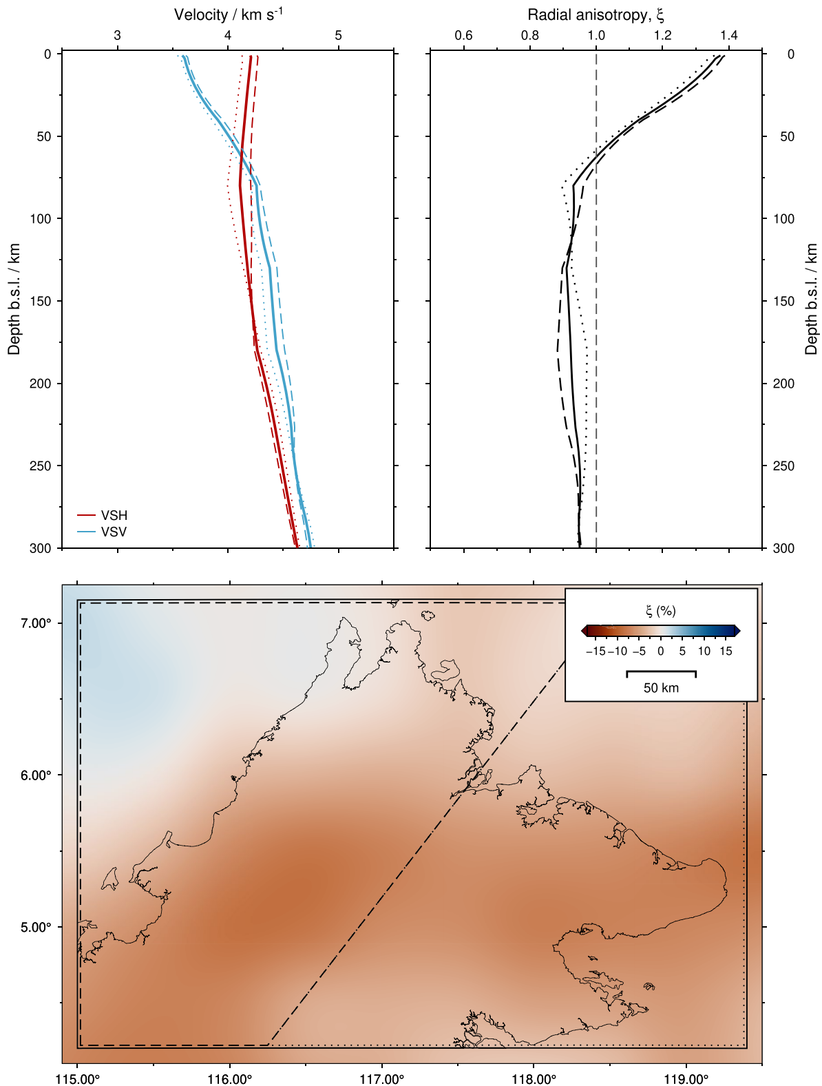
Figure 6. Depth profiles for V_{SH} (red), V_{SV} (blue), and \xi (black) extracted from the recent full-waveform tomographic model of Wehner et al. (2022). The solid lines correspond to the box encompassing the entirety of northern Borneo; the dashed lines correspond to the box encompassing trend 1 (north-west Sabah, striking ~NE-SW); the dotted lines correspond to the box encompassing trend 2 (south-east Sabah, striking ~NW-SE). The lower panel shows the geographic correspondence between the dashed/dotted/solid lines plotted on top of a horizontal slice through a radial anisotropy model derived from the full waveform inversion tomographic model, SASSY21, at 100 km depth (Wehner et al., 2022).
