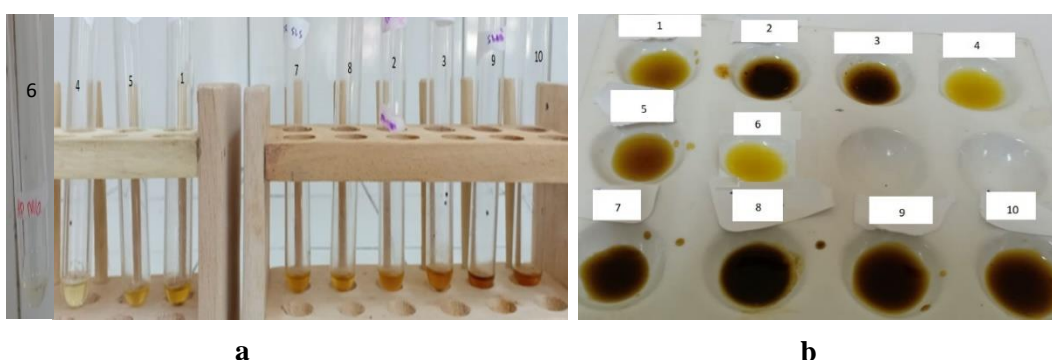
Figure 1. The results of the qualitative test of flavonoids (a) and phenolics (b)
