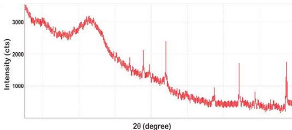
Figure 3. XRD diffraction pattern of rGO
