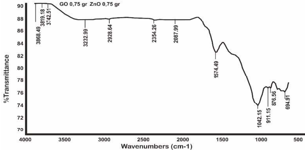
Figure 1. FTIR graphic of rGO
