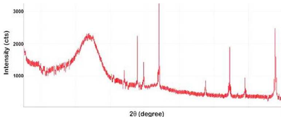
Figure 4. XRD diffraction pattern of rGO-ZnO
