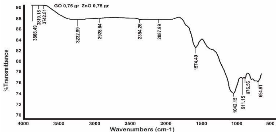
Figure 2. FTIR graphic of rGO-ZnO
