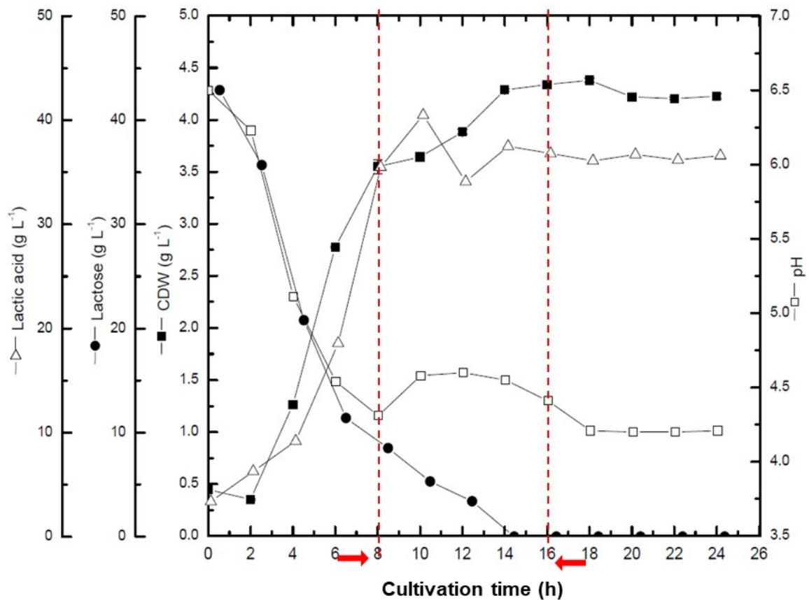
Figure 3. Cell mass production during the batch fermentation of L. reuteri with an integrated anion-exchange resin column ( 10 \text{ g L}^{-1} Amberlite IRA 67). The batch fermentations were performed without a pH control and at an agitation speed of 200 rpm. The fermentation broth was circulated continuously from 8 h of cultivation to 16 h, which are shown with an arrow and dashed line in the graph.
