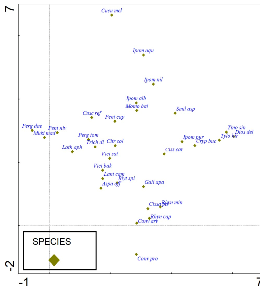
Figure 5. DCA showing the distribution of climber species.
