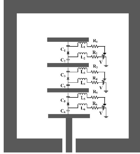
Fig. 4. DC bias network for the PIN diodes.
