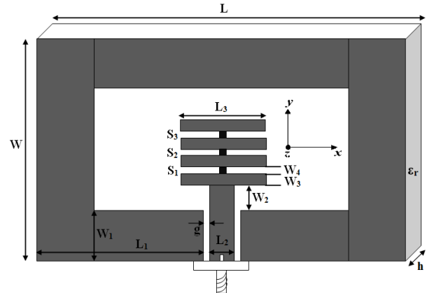
Fig. 1. Geometrical design of the proposed T shaped slot antenna with frequency diversity.
