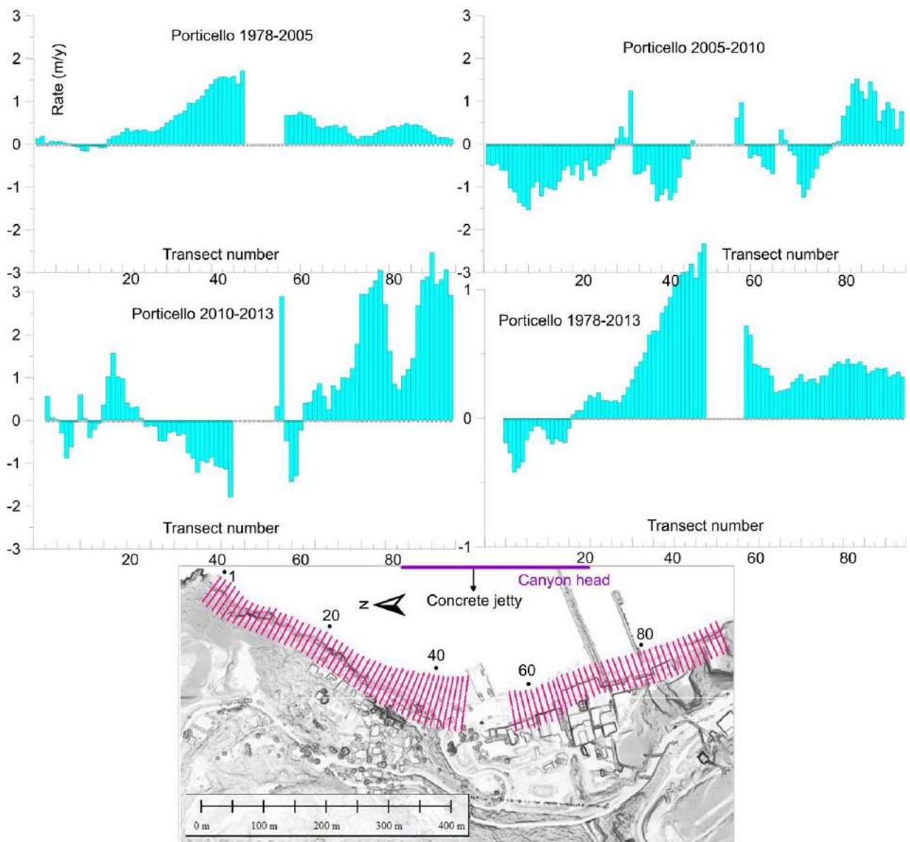
Figure A3. Rate of shoreline displacement for Porticello beach, estimated by means of DSAS along transects spaced 10 m for the different time intervals and for the overall time span of the analysis.
