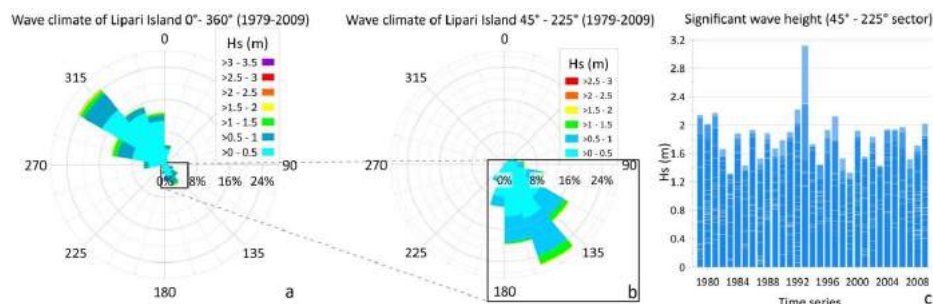
Figure A1. (a) Wave climate of Lipari Island (NOAA hindcasting from 1979 to 2009, [35]) represented as the circular histogram of significant wave height (Hs) related to a position to the north-east of Lipari Island (see text for details). The circular histogram in (b) represents the analysis of wave data only from the sector 45°–225°N and allows the better appreciation of the characteristics of waves from this provenance sector. (c) Time series of significant wave heights from the southeastern sector (45°–225°N).
