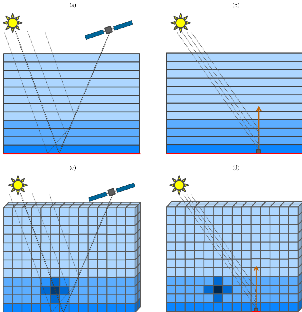
Figure 1. Illustration of the difference between (a, b) 1D-layer and (c, d) 3D-box AMFs for two scenarios with (a, c) downward-looking spaceborne and (b, d) upward-looking ground-based observations. Selected photon paths are shown as dashed lines. The 1D-layer AMFs implicitly assume horizontally uniform atmospheric and surface properties, whereas 3D-box AMFs fully account for both vertical and horizontal variability.
