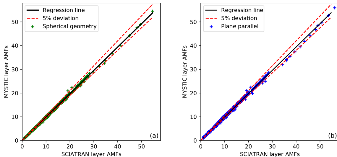
Figure 2. Scatter plots of MYSTIC 1D-layer AMFs computed with (a) spherical and (b) plane-parallel geometries against 1D-layer AMFs computed with SCIATRAN (a) spherical and (b) plane parallel for 67 MAX-DOAS scenarios with 17 layers (1139 points). The solid black lines are the respective regression fits to the points.
