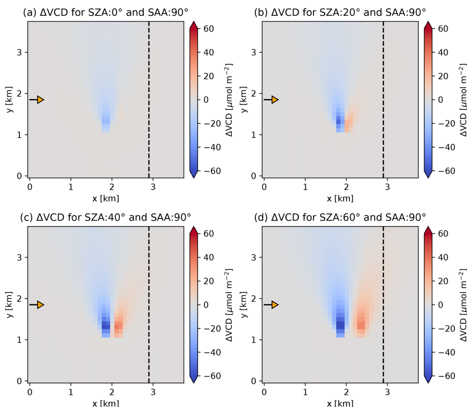
Figure 10. Absolute difference between total VCD from synthetic SCD and 1D box AMF with solar zenith angles (SZAs) of (a) 0°, (b) 20°, (c) 40° and (d) 60° and the true total VCD.
