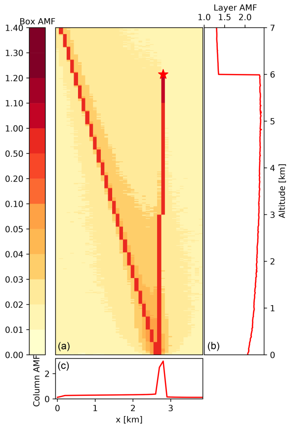
Figure 7. The 3D-box AMFs cross section at y = 1.4 km for the aircraft scenario presented in this section. Aircraft (red star) placed at z = 6 km, x = 2.9 km and y = 1.4 km pointing eastwards. The sun is at SAA = 90^\circ (west) with a SZA of 20^\circ . (b) Vertical profile of horizontally integrated AMFs (1D-layer AMFs). (c) Horizontal profile of vertically integrated AMFs (column AMFs). The default properties are a rural-type aerosol in the PBL, background aerosol above 2 km, spring–summer conditions and a visibility of 50 km.
