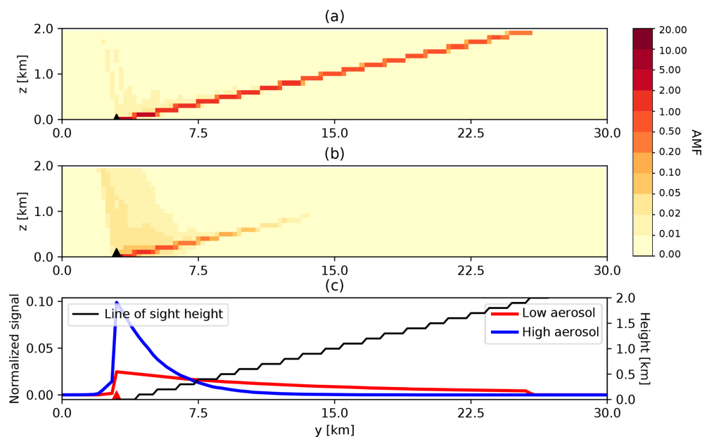
Figure 5. Cross section of 3D-box AMFs for a MAX-DOAS scenario with an instrument (black triangle) at the ground ( z = 0 km, x = 20 km, y = 3 km) pointing northwards and slightly upwards at a viewing angle of 5^\circ . The sun is at an azimuth angle of 344.7^\circ and a zenith angle of 24.6^\circ . The relative azimuth angle between sun and viewing direction is 164.7^\circ . AMFs were simulated with two aerosol scenarios: a rural-type aerosol representative of spring–summer conditions in the aerosol layer (0–2 km), with a visibility of (a) 50 km and a visibility of (b) 10 km and a background aerosol above 2 km. Decay of vertically integrated AMFs with distance to the instrument is visualized (c) for the same scenarios with standard (red) and high aerosols (blue) as in panels (a) and (b). The altitude of the line of sight as a function of distance is shown in black.
