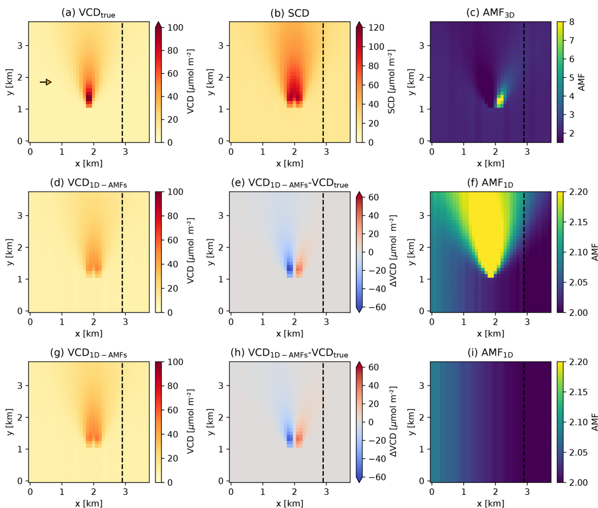
Figure 8. Airborne remote sensing of an \text{NO}_2 plume emitted from a 262.5 m tall stack located at x = 1.9 km and y = 1.3 km. The aircraft flies at an altitude of 6 km from south to north at x = 2.9 km (dashed line) parallel to the plume axis and samples the plume in the across-track direction. The sun is located in the west (small arrow in panel a ) at a zenith angle of 40^\circ . The panels show (a) simulated (true) \text{NO}_2 VCDs, (b) synthetic SCDs computed from the simulated \text{NO}_2 distribution by applying 3D-box AMFs and (c) 3D-box AMFs computed with MYSTIC. The second row shows (d) VCDs calculated from the SCDs using 1D-layer AMFs and the “true” \text{NO}_2 profile above the ground pixel pointed by the instrument, (e) the difference between calculated and true VCDs, and (f) total AMFs from the MYSTIC 1D module. The third row (g–i) shows the same as panels (d)–(f) but using the background \text{NO}_2 profile to compute AMFs.
