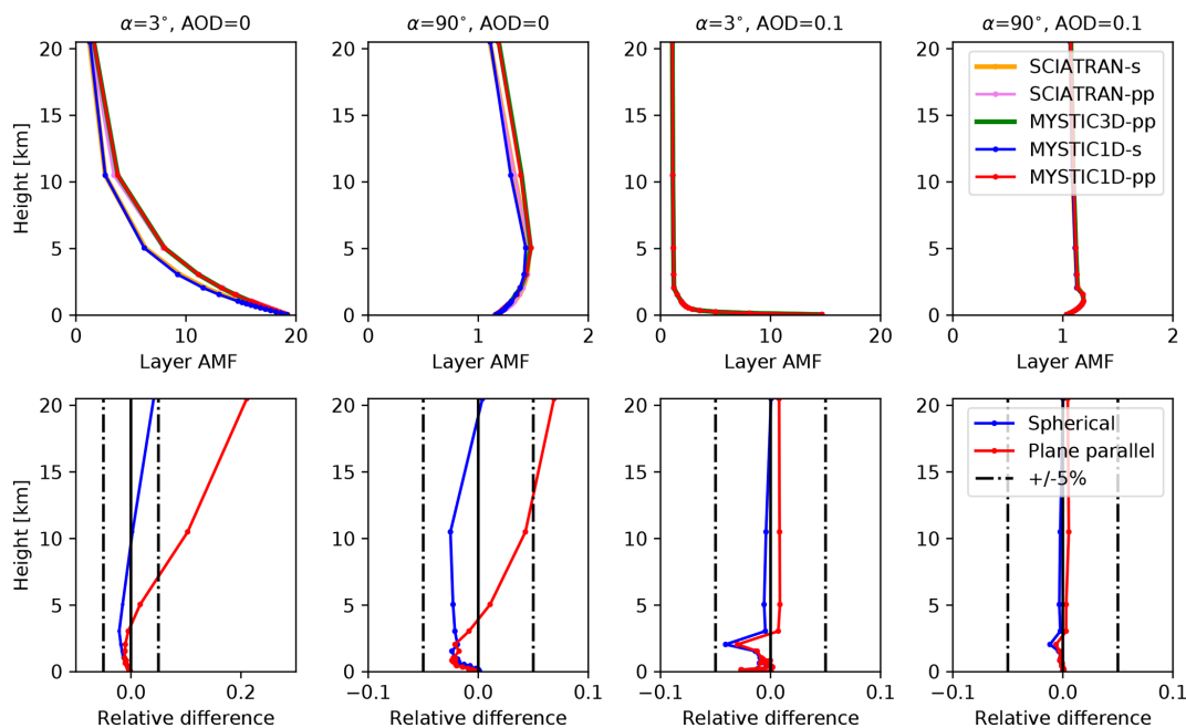
Figure 3. Upper row: MAX-DOAS AMF profiles for MYSTIC 1D spherical geometry (s), 1D plane-parallel geometry (pp) and 3D plane-parallel geometry (pp) for two selected elevation angles of 3 and 90°, a SZA of 20°, with and without aerosol for radiation at 577 nm. Corresponding profiles computed with the SCIATRAN RTM are shown for comparison. Lower row: profile of relative differences of MYSTIC and SCIATRAN results in spherical (s) and plane-parallel geometry (pp) (Wagner et al., 2007).
