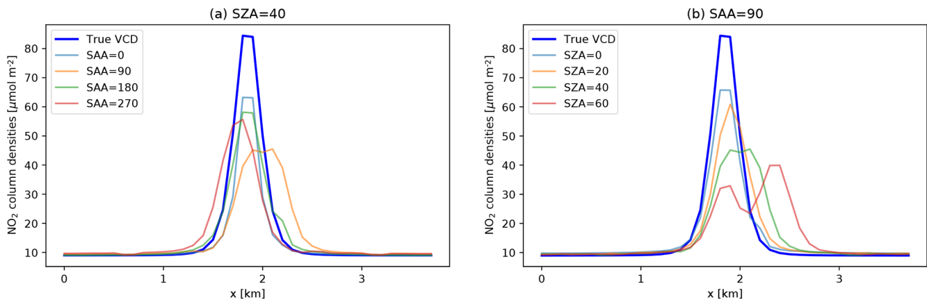
Figure 12. Plume VCD cross section at y = 1.6 km (0.3 km downstream of the plume) for (a) the sun at \text{SZA} = 40^\circ with different SAAs and (b) for the sun in the west with different SZAs.
