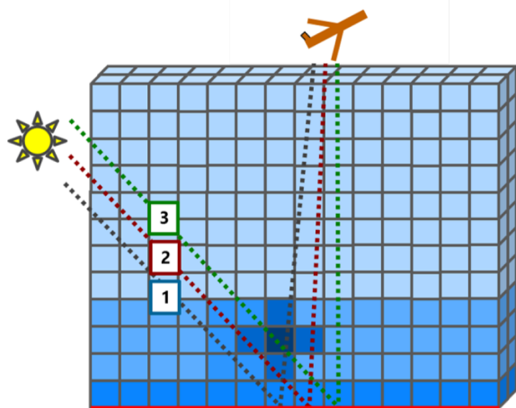
Figure 9. Schematic of the across-track measurement by the aircraft measuring a \text{NO}_2 plume (dark blue corresponding to high \text{NO}_2 concentrations) with three main photon paths for three measurement geometries (1, 2, 3).
