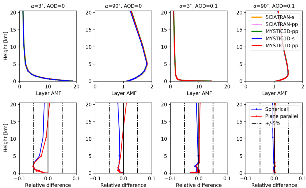
Figure 4. Upper row: MAX-DOAS AMF profiles for MYSTIC 1D spherical geometry (s), 1D plane-parallel geometry (pp) and 3D plane-parallel geometry (pp) for two selected elevation angles of 3 and 90°, a SZA of 20°, with and without aerosol for radiation at 360 nm. Corresponding profiles computed with the SCIATRAN RTM are shown for comparison. Lower row: profile of relative differences of MYSTIC and SCIATRAN results in spherical (s) and plane-parallel geometry (pp) (Wagner et al., 2007).
