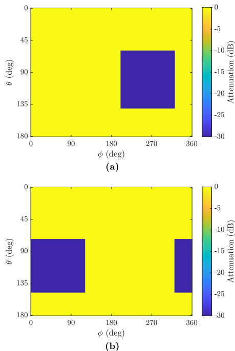
FIGURE 6. Stereographic projection of 3GPP's self-blocking attenuation region. (a) Portrait mode. (b) Landscape mode.
