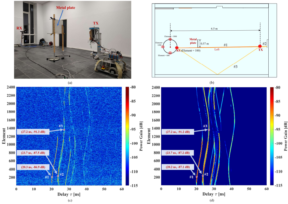
Fig. 2. Empty room scenario: a) RX view in the empty room scenario; b) Ray trajectories; c) Power-delay-element measurement result; d) Power-delay-element simulation result.
