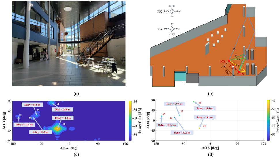
Fig. 3. Spacious hall scenario: a) Photograph in the hall scenario; b) Ray trajectories; c) Power-AOA-AOD measurement result; d) Power-AOD-AOA simulation result.
