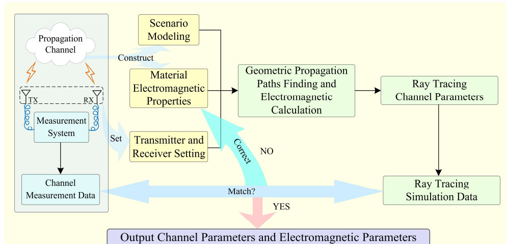
Fig. 1. Flowchart of measurement-calibrated RT channel simulation.
