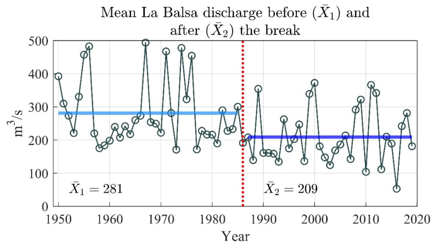
Figure 2. Mean La Balsa discharge time series from November to January (NDJ) during the 1950–2019 period (solid line). According to the Pettitt test, the vertical red dashed line indicates the break year (1986), significant at the 0.05 significance level. The two horizontal lines represent the mean discharge value before ( \bar{X}_1 ) and after ( \bar{X}_2 ) the break.
