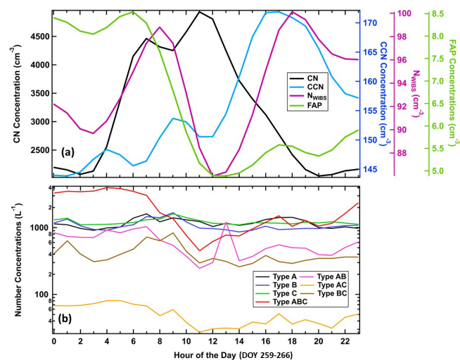
Figure 3. (a) Hourly concentrations of CN (black curve) and CCN at 0.3 % supersaturation (solid blue curve), N_{WIBS} (magenta) and FAP (green) concentrations. (b) Hourly concentrations of the seven types of FAPs.
