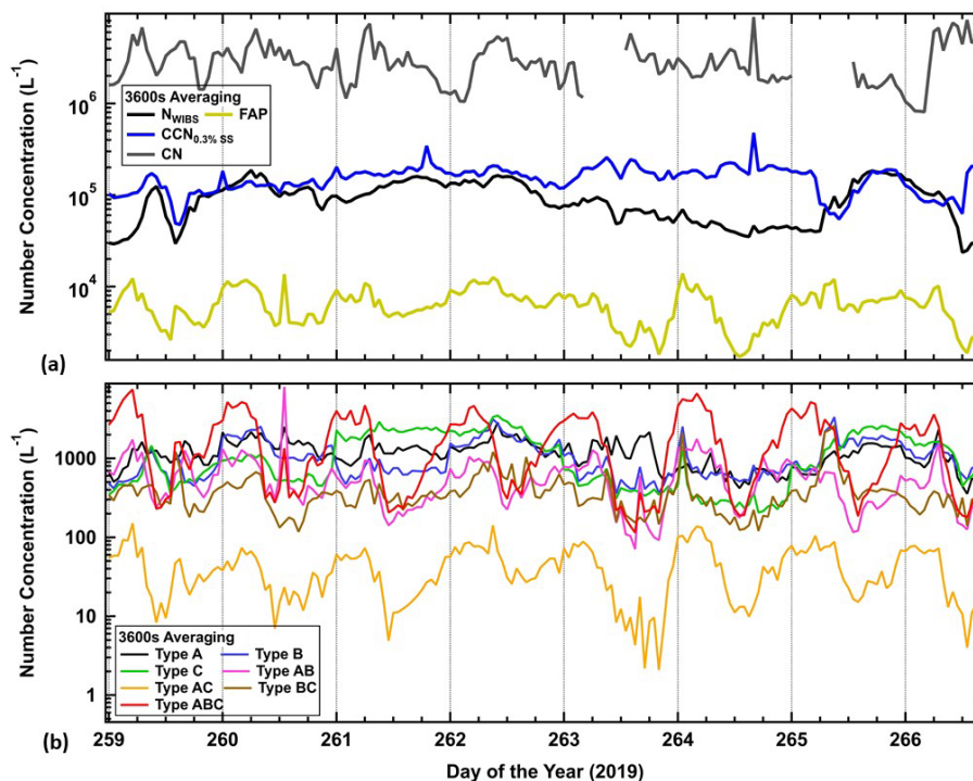
Figure 2. Time series of the number concentrations of (a) CN, CCN, N_{WIBS} and FAPs as well as of (b) FAP types A, B, C, AB, AC, BC and ABC. The gaps in time in the CN concentrations were when the CPC was offline.
