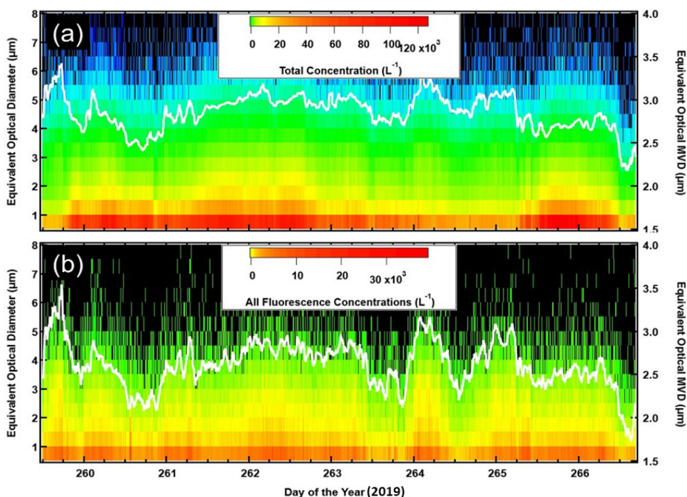
Figure 4. Time series of (a) total and (b) fluorescent particle size distributions measured by WBS for the period from 16 to 23 September (DOY 259–266) 2019. The white curves are the average median volume diameters (MVDs).
