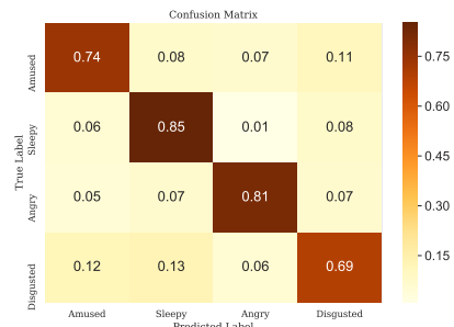
Figure 5: Proposed method
