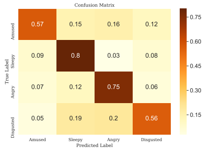
Figure 6: Seq2Seq-EVC
