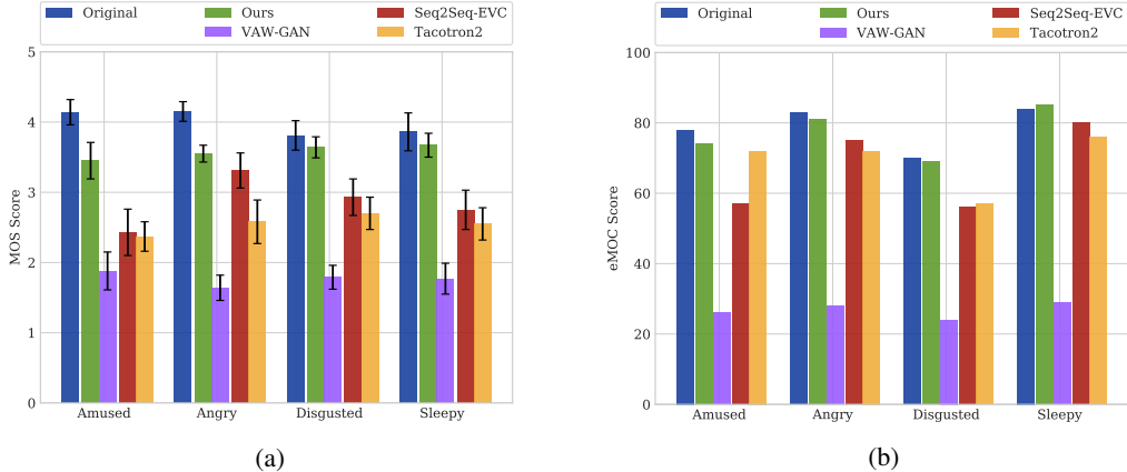
Figure 3: Results for a subjective evaluation of our model against baselines. Sub-figure (a) reports the Mean-Opinion-Score (MOS), measuring the perceived audio-quality. We report mean scores with a Confidence Interval of 95%. Sub-figure (b) reports the Emotion-Mean-Opinion-Classification (eMOC) score, measuring the perceived emotion. We report mean scores for each emotion (chance level: 25%).
