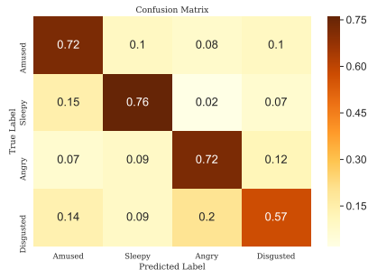
Figure 7: Tacotron2
