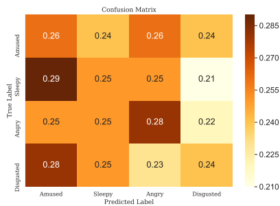
Figure 8: VAW-GAN
