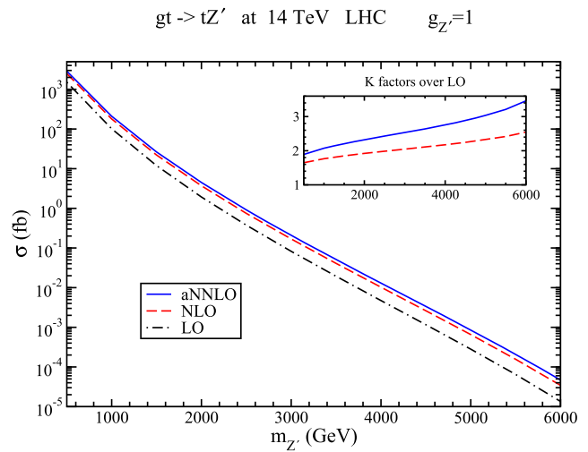
Fig. 20 Total cross section for the gt \rightarrow tZ' process at the LHC 13 TeV (left) and 14 TeV (right). LO, NLO and NNLO calculations are obtained using NNPDF3.1 NNLO n_f = 6 PDFs
