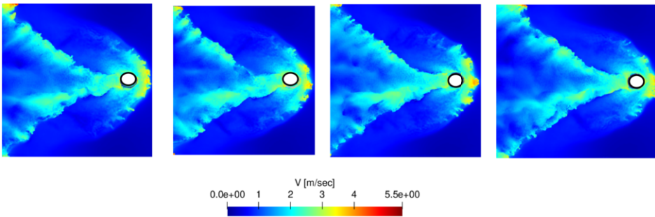
Figure 3. Turbulent wake for the four snorkel designs. Left to right, S#1 to S#4. t \cdot U/D = 100 .
