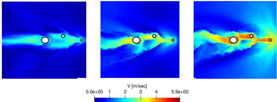
Figure 5. Turbulent wake for staggered masts configuration. Left to right: Fn_D = [1.43; 2.14; 2.86] . t \cdot U/D = 100 .
