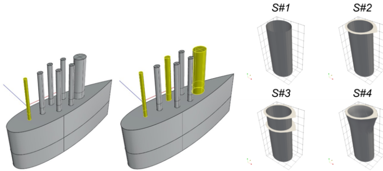
Figure 1. Mast's configurations. Left to right: periscope alone; periscope, antenna and snorkel (staggered); different snorkel designs.
