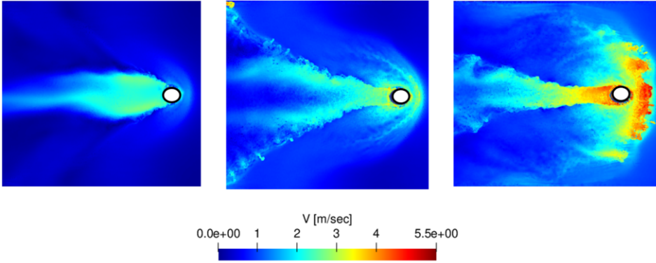
Figure 2. Turbulent wake for the periscope. Left to right: Fn_D = [1.43; 2.14; 2.86] . t \cdot U/D = 100 .
