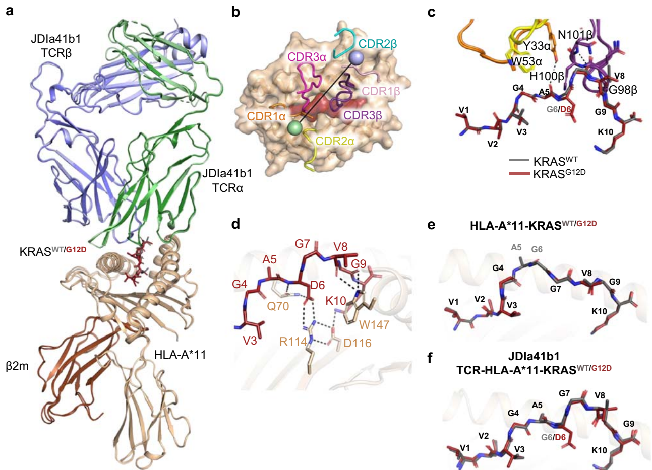
Fig. 2 | The JDla41b1 TCR adopts a virtually identical binding mode in complex with HLA-A*11-KRAS G12D and HLA-A*11-KRAS WT . a Superposition of JDla41b1-HLA-A*11-KRAS WT (PDB 70W5) and JDla41b1-HLA-A*11-KRAS G12D (PDB 70W6) complexes. The HLA, \beta 2m, JDla41b1 TCR \alpha , and TCR \beta are coloured in wheat, brown, green, and blue respectively. The darker shades of green and blue correspond to the JDla41b1 TCR in the JDla41b1-HLA-A*11-KRAS G12D complex. The KRAS WT and KRAS G12D peptides are coloured in grey and maroon respectively. b Top view of the JDla41b1-HLA-A*11-KRAS G12D complex (PDB 70W6). The HLA and KRAS G12D peptide are shown in surface representation and the CDRs are shown in cartoon tube representations. The
