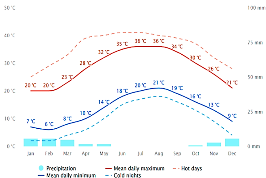
Figure 2. Climate parameters of the studied area.
