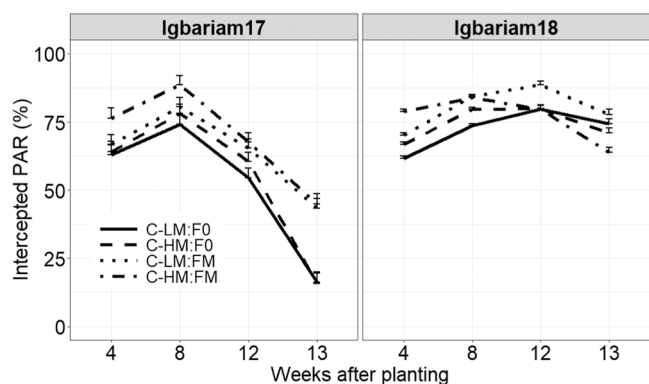
Fig. 6. Intercepted PAR over time, as affected by maize planting density and NPK application in cassava-maize intercropping system at Igbariam in Igbariam17 and Igbariam18. C: cassava at 12,500 ha -1 ; LM: low density maize (20,000 ha -1 ); HM: high density maize (40,000 ha -1 ); F0: no fertilizer applied; FM: fertilizer application at 90 kg N ha -1 , 20 kg P ha -1 and 37 kg K ha -1 . Error bars represent standard errors of the mean.
