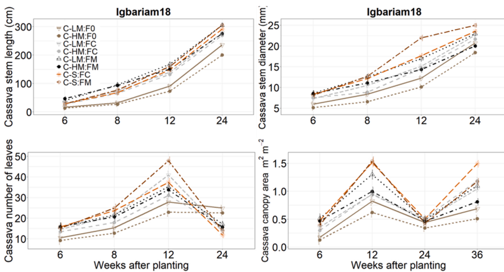
Fig. 5. Cassava stem length, stem diameter, leaf production, and canopy area over time, as affected by maize planting density and NPK application in cassava-maize intercropping system at Igbariam18. C: cassava at 12,500 ha -1 ; S: sole crop; LM: low density maize (20,000 ha -1 ); HM: high density maize (40,000 ha -1 ); F0: no fertilizer applied; FM: fertilizer application at 90 kg N ha -1 , 20 kg P ha -1 and 37 kg K ha -1 ; FC: fertilizer application at 75 kg N ha -1 , 20 kg P ha -1 and 90 kg K ha -1 . Error bars represent standard errors of the mean.
