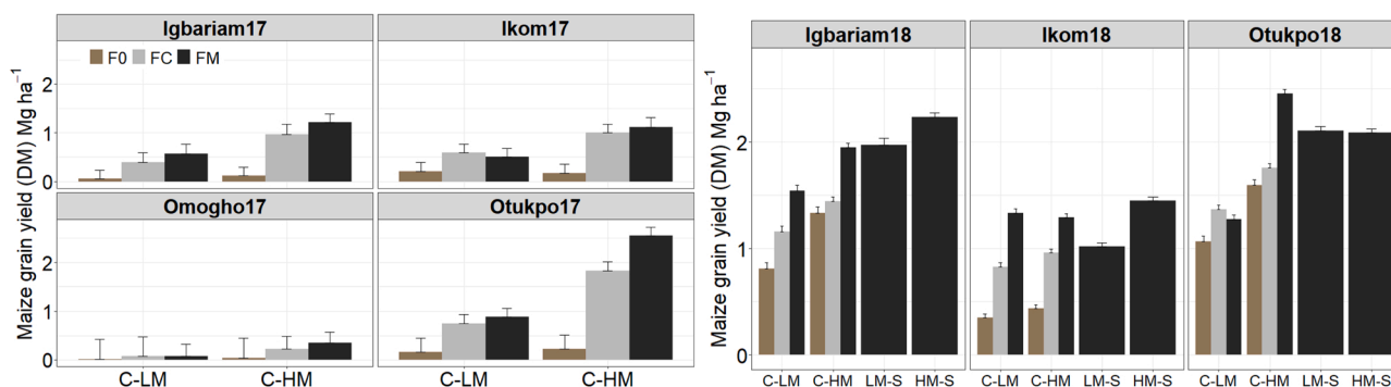
Fig. 9. Maize grain yield as affected by maize planting density and NPK application in cassava-maize cropping systems at Igbariam, Ikom, Omogho, and Otukpo in 2017 and 2018 (except Omogho due to trial pilferage). C: cassava at 12,500 ha -1 ; LM: low density maize (20,000 ha -1 ); HM: high density maize (40,000 ha -1 ); S: sole crop; F0: no fertilizer applied; FM: fertilizer application at 90 kg N ha -1 , 20 kg P ha -1 and 37 kg K ha -1 ; FC: fertilizer application at 75 kg N ha -1 , 20 kg P ha -1 and 90 kg K ha -1 . Error bars represent standard errors of the mean.
