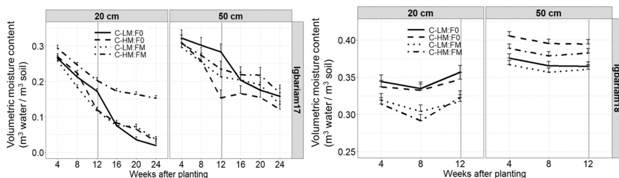
Fig. 8. Soil volumetric water content over time and depths as affected by maize planting density and NPK application in cassava-maize intercropping systems at Igbariam17 and Igbariam18. C: cassava at 12,500 ha -1 ; LM: low density maize (20,000 ha -1 ); HM: high density maize (40,000 ha -1 ); F0: no fertilizer applied; FM: fertilizer application at 90 kg N ha -1 , 20 kg P ha -1 and 37 kg K ha -1 . Error bars represent standard errors of the mean. The vertical line shows the day of maize harvest.
