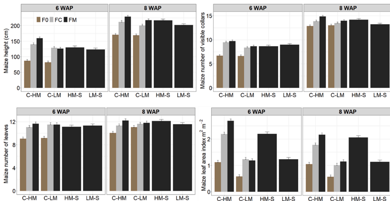
Fig. 3. Maize height, visible collars, leaf production, and leaf area index at 6 and 8 weeks after planting (WAP) as affected by maize planting density, and NPK application in cassava-maize intercropping systems at Igbariam18 in 2018. C: cassava at 12,500 ha -1 ; S: sole crop; LM: low density maize (20,000 ha -1 ); HM: high density maize (40,000 ha -1 ); FO: no fertilizer applied; FM: fertilizer application at 90 kg N ha -1 , 20 kg P ha -1 and 37 kg K ha -1 ; FC: fertilizer application at 75 kg N ha -1 , 20 kg P ha -1 and 90 kg K ha -1 . Error bars represent standard errors of the mean.
