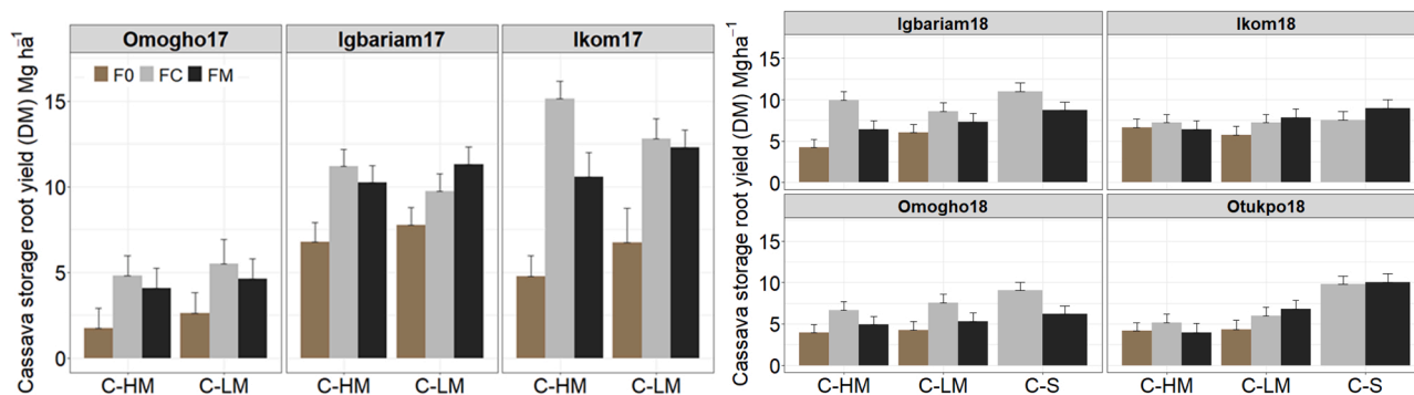
Fig. 10. Cassava storage root yield (in DM) as affected by maize planting density and NPK application in cassava-maize cropping systems at Igbariam, Ikom, Omogho, and Otukpo in 2017 (except Otukpo due to trial pilferage) and 2018. C: cassava at 12,500 ha -1 ; LM: low density maize (20,000 ha -1 ); HM: high density maize (40,000 ha -1 ); S: sole crop; F0: no fertilizer applied; FM: fertilizer application at 90 kg N ha -1 , 20 kg P ha -1 and 37 kg K ha -1 ; FC: fertilizer application at 75 kg N ha -1 , 20 kg P ha -1 and 90 kg K ha -1 . Error bars represent standard errors of the mean.
