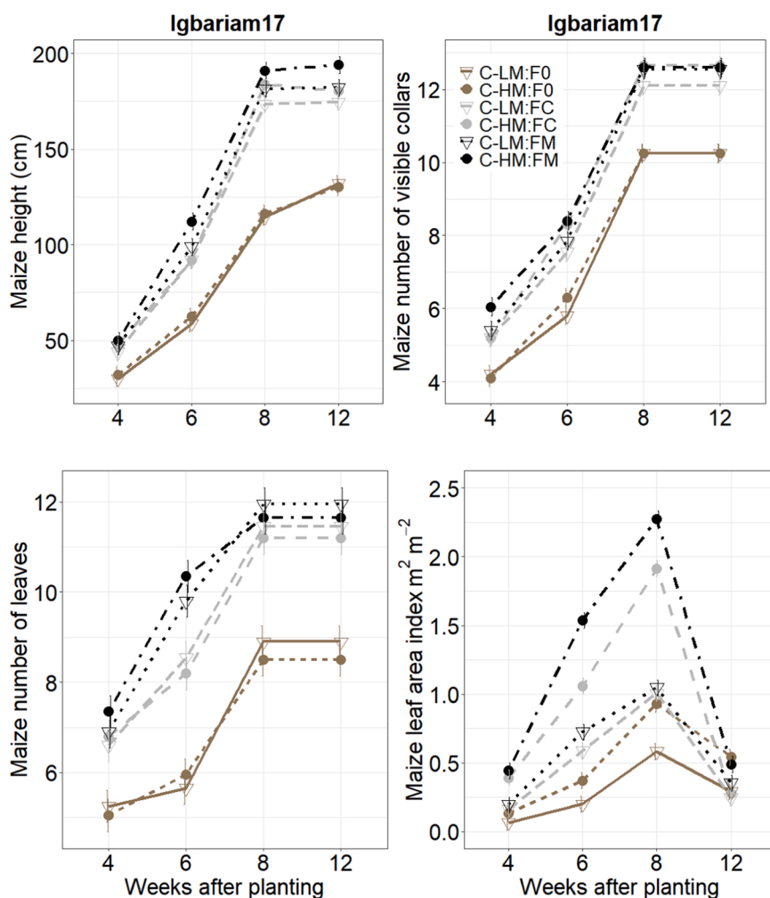
Fig. 2. Maize height, visible collars, leaf production, and leaf area index over time as affected by maize planting density and NPK application in cassava-maize intercropping systems at Igbariam17 in 2017. C: cassava at 12,500 ha -1 ; LM: low density maize (20,000 ha -1 ); HM: high density maize (40,000 ha -1 ); F0: no fertilizer applied; FM: fertilizer application at 90 kg N ha -1 , 20 kg P ha -1 and 37 kg K ha -1 ; FC: fertilizer application at 75 kg N ha -1 , 20 kg P ha -1 and 90 kg K ha -1 . Error bars represent standard errors of the mean.
