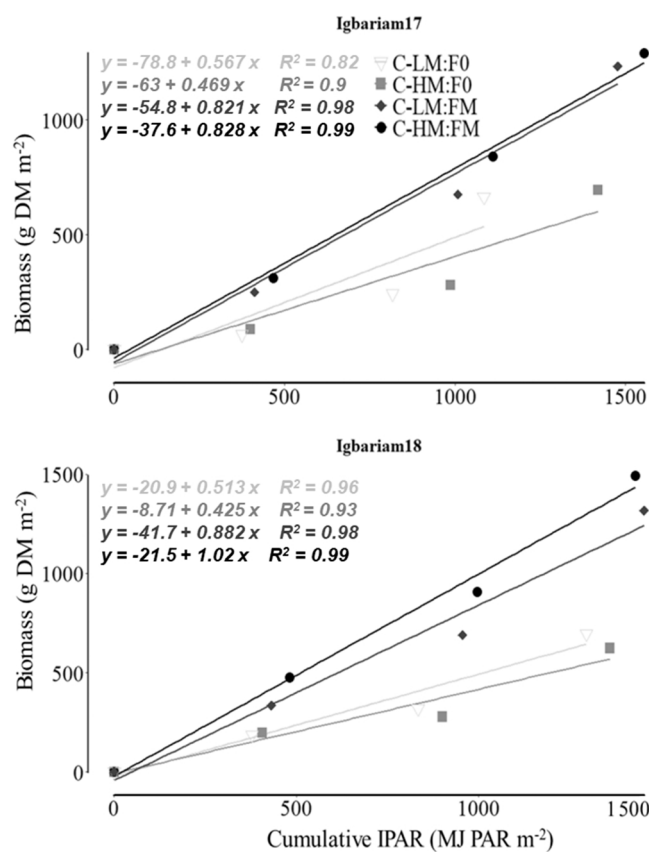
Fig. 7. Relationship between the combined cassava and maize biomass yields over time, the cumulative amount of IPAR, and the regression lines indicating radiation use efficiencies (RUE = the slope of the lines) for each intercrop treatment in cassava-maize intercropping systems at Igbariam17 and Igbariam18 in 2017 and 2018. C: cassava at 12,500 ha -1 ; LM: low density maize (20,000 ha -1 ); HM: high density maize (40,000 ha -1 ); F0: no fertilizer applied; FM: fertilizer application at 90 kg N ha -1 , 20 kg P ha -1 and 37 kg K ha -1 .
