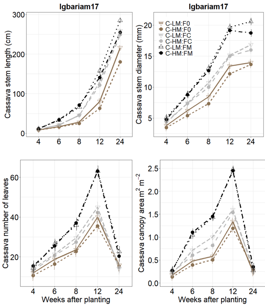
Fig. 4. Cassava stem length, stem diameter, leaf production, and canopy area over time, as affected by maize planting density and NPK application in cassava-maize intercropping system at Igbariam17. C: cassava at 12,500 ha -1 ; LM: low density maize (20,000 ha -1 ); HM: high density maize (40,000 ha -1 ); F0: no fertilizer applied; FM: fertilizer application at 90 kg N ha -1 , 20 kg P ha -1 and 37 kg K ha -1 ; FC: fertilizer application at 75 kg N ha -1 , 20 kg P ha -1 and 90 kg K ha -1 . Error bars represent standard errors of the mean.
