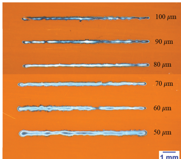
Fig. 6 Printed lines on polyimide using Waveform1 at stage velocity 30 \text{ mm s}^{-1} and drop spacing 50 \mu\text{m} , 60 \mu\text{m} , 70 \mu\text{m} , 80 \mu\text{m} , 90 \mu\text{m} and 100 \mu\text{m} .
