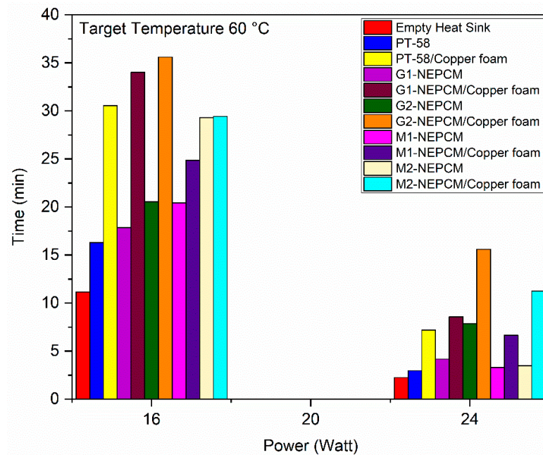
Figure 20. Time to attain target temperature of 60 °C for heat sink filled with PCM, NEPCM and NEPCM/copper foam composites.
