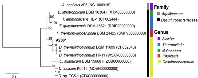
FIG 1 Phylogenomic tree of Desulfurobacterium sp. strain AV08 (marked with an asterisk) and related Desulfurobacteriaceae and Aquificaceae (outgroup) family strains. All available Desulfurobacteriaceae genomes with >97% genome completeness are included. Families and genera are indicated by color.
