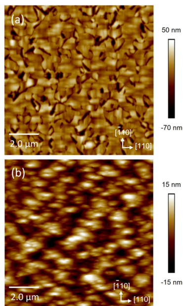
Fig. 2 10 \times 10 \mu\text{m}^2 AFM measurements of a 1 \mu\text{m} GaAs surface grown on Si (001) substrates (a) without and (b) with the growth-during-ramp method.
