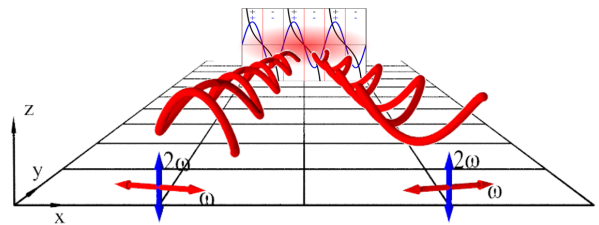
FIG. 1. Schematic plot of two non-collinear laser beams, each consisting of \omega - 2\omega orthogonally polarized linear fields; \omega is polarized on the x-y plane and 2\omega along the z-axis. Both beams propagate towards the atom in the focus region (red-shaded ellipse). The resultant electric field has chirality (square inset) that changes along the x-axis in the focus region.
