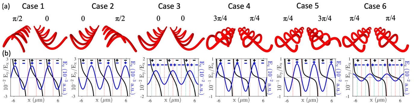
FIG. 2. (a) Schematic plots of six combinations of two non-collinear beams; (b) change of sign of E_y/E_x (black) and E_z (blue) along the x axis in the focus region, at y=z=0 , t=T/50 . For each case, above beams 1 and 2, we denote \phi_1^{2\omega} - \phi_1^\omega and \phi_2^{2\omega} - \phi_2^\omega from left to right.
