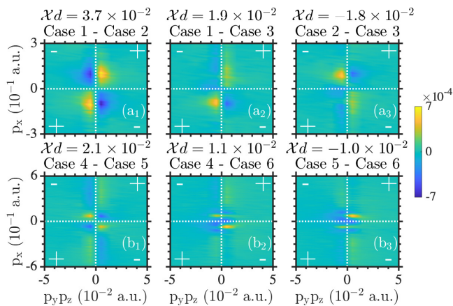
FIG. 4. Probability distribution P^{m,n}(p_x, p_y, p_z) . The m,n indexes are 1,2 for Case 1-Case 2, 1,3 for Case 1-Case 3, 2,3 for Case 2-Case 3, 4,5 for Case 4-Case 5, 4,6 for Case 4-Case 6 and 5,6 for Case 5-Case 6. The sign in each quadrant corresponds to the sign of \mathbf{p}_x \cdot (\mathbf{p}_y \times \mathbf{p}_z) in this quadrant.
