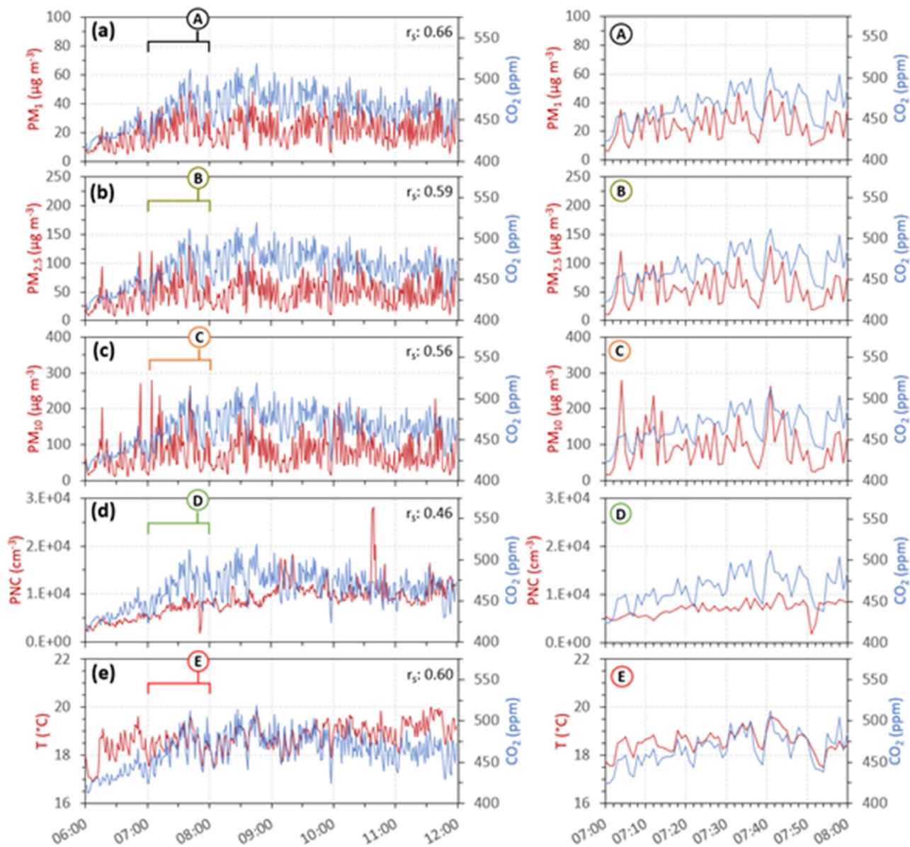
Fig. 7. Temporal variation (1-min resolution) between 06:00 and 12:00 h (October 01, 2020) for (a) PM 1 ; (b) PM 2.5 ; (c) PM 10 ; (d) PNC; and (e) Temperature. Spearman correlation ( r_s ) between each variable with CO 2 is indicated in the top right corner of each panel. ACH obtained for this day is ( 0.23 \text{ h}^{-1} ). Upper case letters A-E represent the selected time-window range (07:00–08:00 h).
