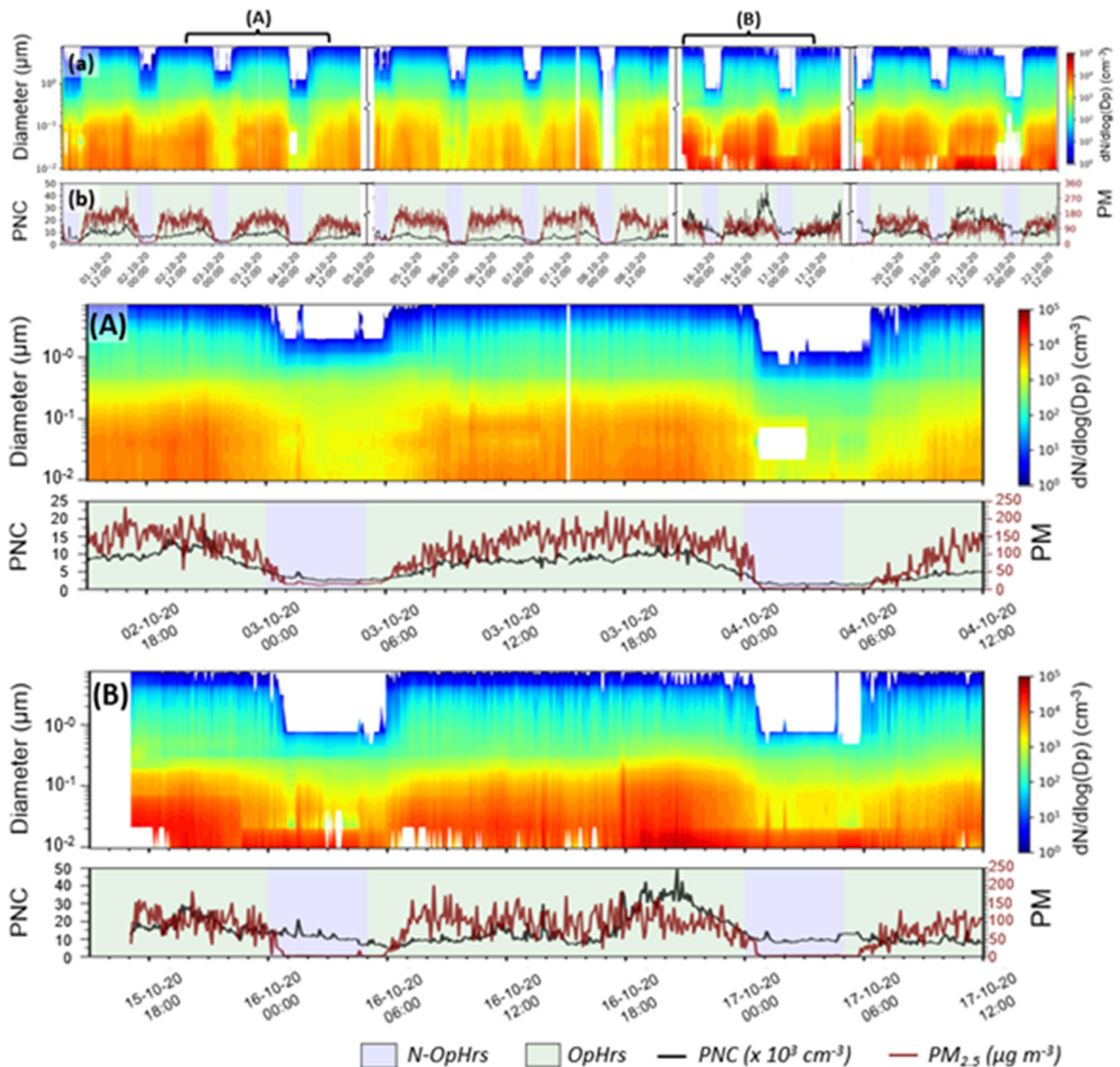
Fig. 6. Temporal variation of (a) PNDs, (b) PNCs and PM_{2.5} during field measurements (top figure). Upper case letters A–B represent two selected time ranges. PM_{2.5} was obtained using the ELPI+ macro file assuming a particle density of 1 \text{ g cm}^{-3} . Blue and green shaded areas represent the underground non-operational (N-OpHrs) and operational hours (OpHrs), respectively.
