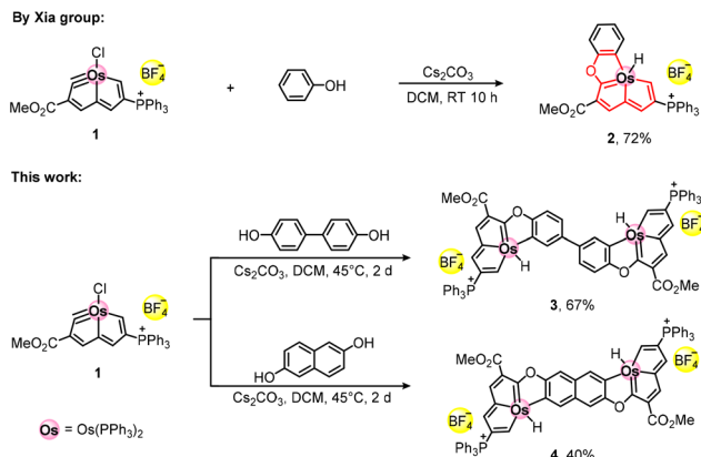
Scheme 1 Syntheses of 2–4.
