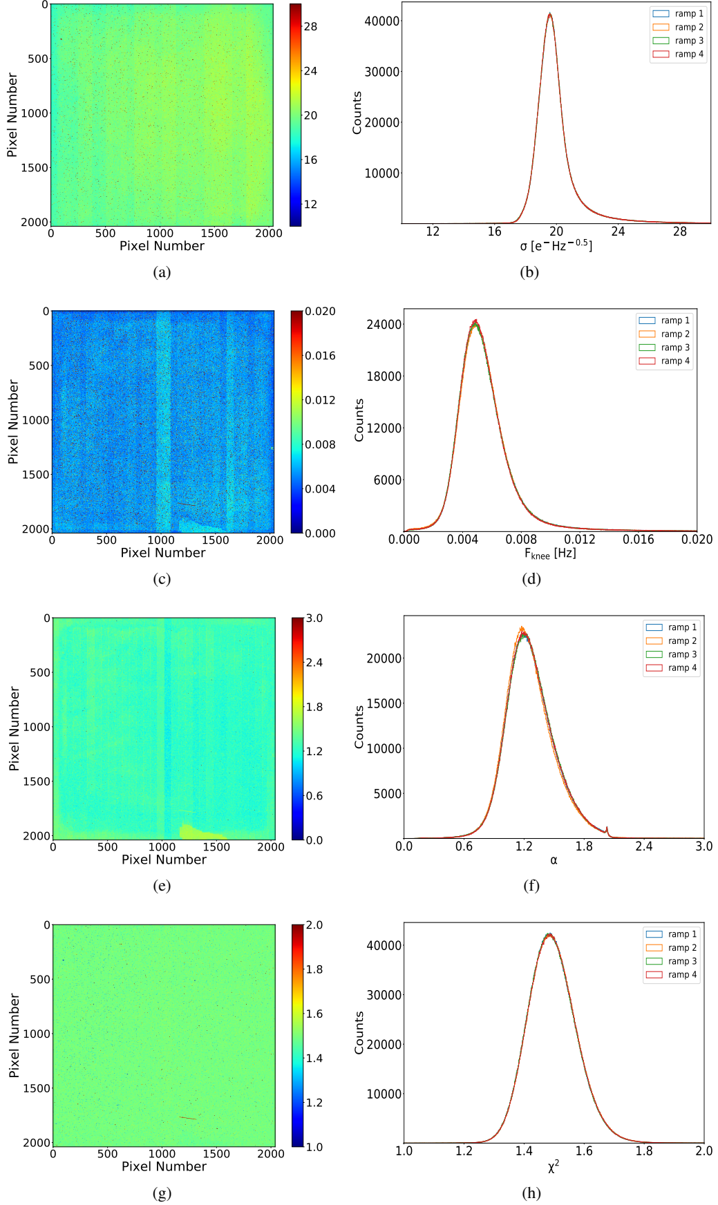
Figure 3: (1/f)^\alpha -like model best-fit parameters \sigma , f_{\text{knee}} and \alpha for the photosensitive pixels of one of the NISP detectors tested. Panels (a), (c), (e) and (g) are maps representing the best-fit values for the three parameters and the \chi^2/N_{\text{dof}} for the 2040 \times 2040 photosensitive pixels of the detector for a single ramp. Panels (b), (d), (f) and (h) show the 1D distribution for the same best-fit parameters of 4 ramps of the same detector, and the \chi^2/N_{\text{dof}} , respectively. See main text for details.
