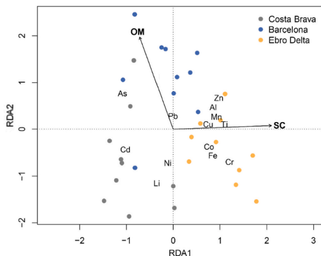
Fig. 2. Redundancy analysis (RDA) on the tissue levels of metallic elements in N. norvegicus from three locations constrained by the physicochemical parameters of near-bottom waters and sediments, from which the content of organic matter (OM) and the percentage of silt and clay (SC) were selected as the most significant explanatory variables for the ordination. For interpretation of the references to colour in the legend, the reader is referred to the web version of the article. (For interpretation of the references to colour in this figure legend, the reader is referred to the Web version of this article.)
