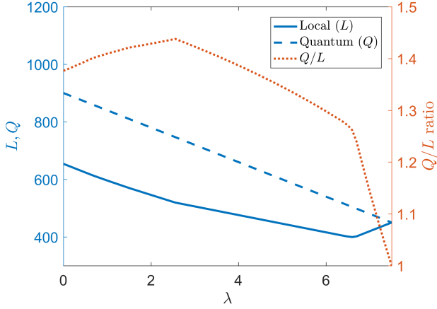
Figure 2: The Q/L ratio (red dots) in the function of \lambda for the Platonic Bell inequality defined by the coefficients (19), where \vec{A}_i are the vertices of the halved tetraplex. The functions Q (blue dashed line) and L (blue solid line) are also plotted against \lambda . The maximum ratio Q/L = 1.4377579 - \epsilon is obtained at \lambda = 23/9 , where \epsilon = 4 \times 10^{-6} . The value 1.4377579 is analytically given by 70/(5+27\phi) , where \phi = (1+\sqrt{5})/2 is the golden ratio.
