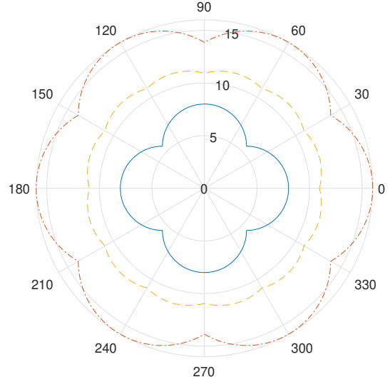
Figure 1: Dependence of the local bound on the relative orientation of the two regular polygons used to construct the Bell inequality. The solid, the dash-dotted and the dashed line correspond to two squares, two hexagons and a square and a hexagon, respectively. At zero angle (at least) two vertices align.
