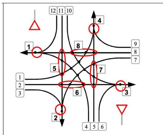
Figure 3. Conflict at the Unsignalized Intersections [15]
