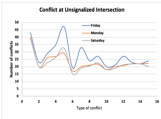
Figure 10. Graph of Conflicts Occurring at Unsignalized Intersections
