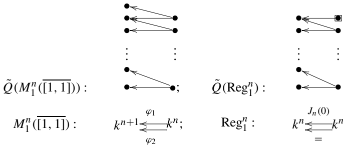
Fig. 2 Coefficient-quiver of Q_{1,1} -representations
