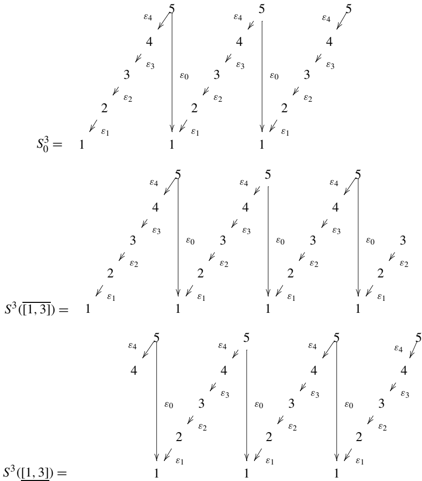
Fig. 1 The coefficient-quiver of \text{Reg}_4^3(0) , M_4^3(\overline{[1, 3]}) and M_4^3(\underline{[1, 3]}) respectively
