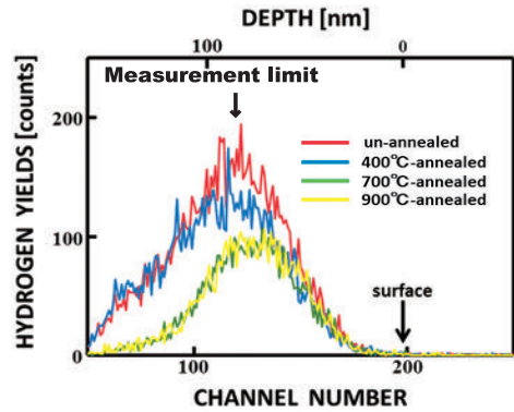
Fig. 3 The residual hydrogen in un-annealed, 400, 700 and 900°C-annealed GaN evaluated by ERDA using 1.8 MeV ^4\text{He}^+ beam. ERDA measured using 1.8 MeV - ^4\text{He}^+ ion beam can evaluate hydrogen until about 90 nm in depth due to the energy loss of the analytical beam in the solid. The arrow above the ERDA peak indicates the limit of the quantitative calculation of the hydrogen concentrations.
