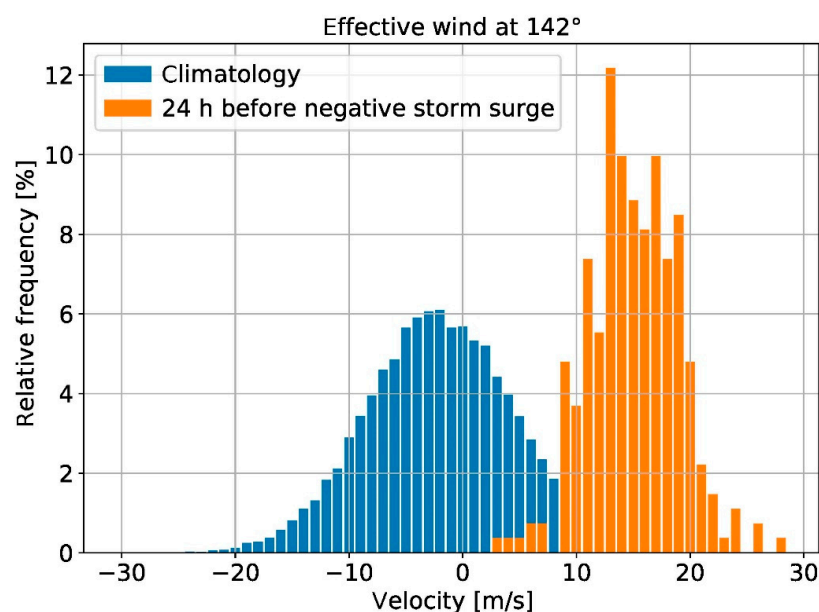
Figure 11. Distribution of the effective wind at 142^\circ for the whole time period 1950–2019 (climatology, blue) and for the 24 h before the respective 271 ELWs (orange).
