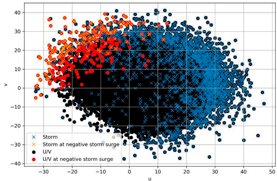
Figure A1. Distribution of the U and V components of the geostrophic wind from the LWT classification for daily means (black) and for the 24-h mean before an ELW (red). Marked also is whether a gale was present at that time (blue and yellow 'x', respectively).
