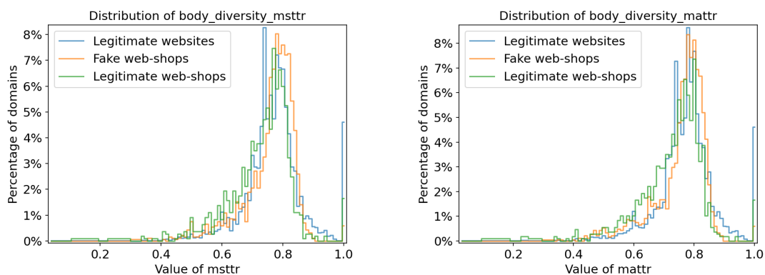
(c) Distribution of the msttr computed on the body text of the HTML pages. (d) Distribution of the mattr computed on the body text of the HTML pages.
