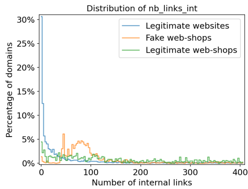
(a) Fake web-shops tend to have more internal links than legitimate websites.
