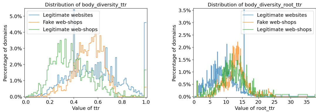
(a) Distribution of the ttr computed on the body text of the HTML pages. (b) Distribution of the root_ttr computed on the body text of the HTML pages.
