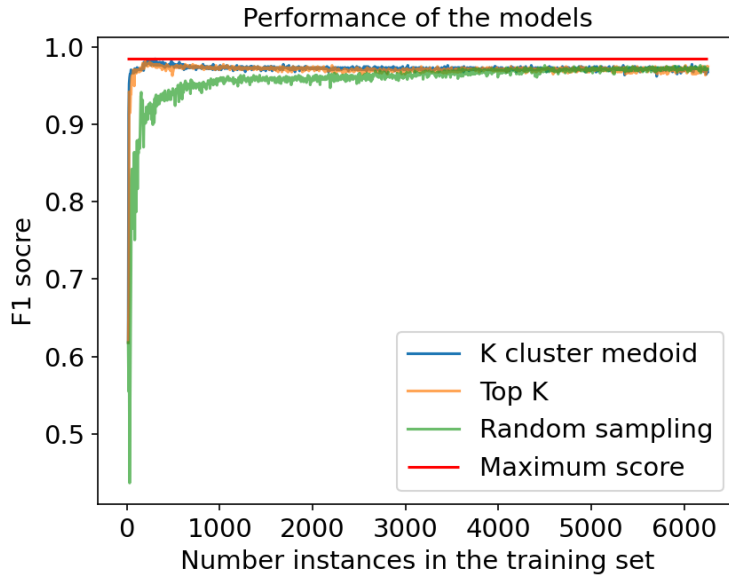
Figure 5.1: F1 score of the different learners as more instances are added to their training set. Both Top K and K Cluster Medoid perform better than random sampling .
