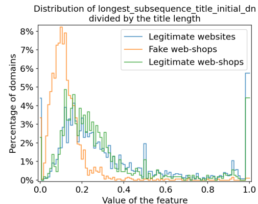
(f) Distribution of the longest_subsequence_title_initial_dn divided by the length of the title of the HTML computed on the baseline dataset.
