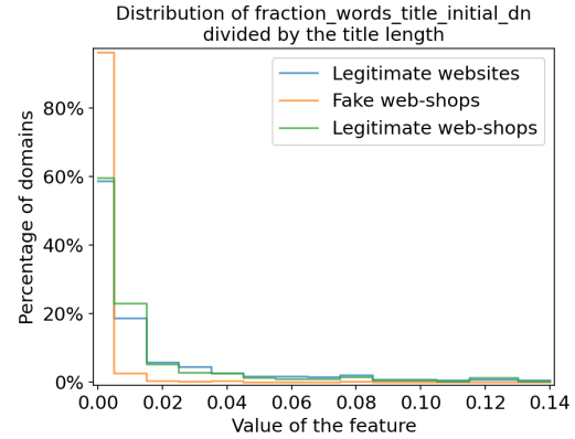
(b) Distribution of the fraction_words_title_initial_dn divided by the length of the title of the HTML computed on the baseline dataset.
