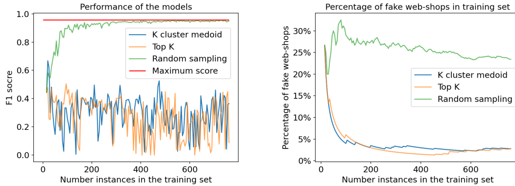
(a) F1 score of the different learners as more instances are added in their training set. (b) Percentage of fake web-shops in the labeled dataset of the learners.
