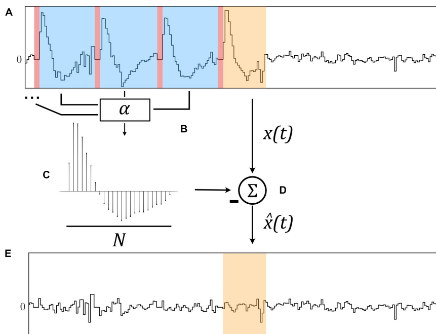
FIGURE 1 The Template Subtraction (TS) algorithm identifies stimulation artifacts from the original signal x(t) [(A), in blue] immediately following neurostimulation [(A), in red] and averages them using exponential filters (B) to form an artifact template (C). This template is subtracted from a newly-identified artifact [(D), in orange] to yield an estimated artifact-free signal \hat{x}(t) (E).
