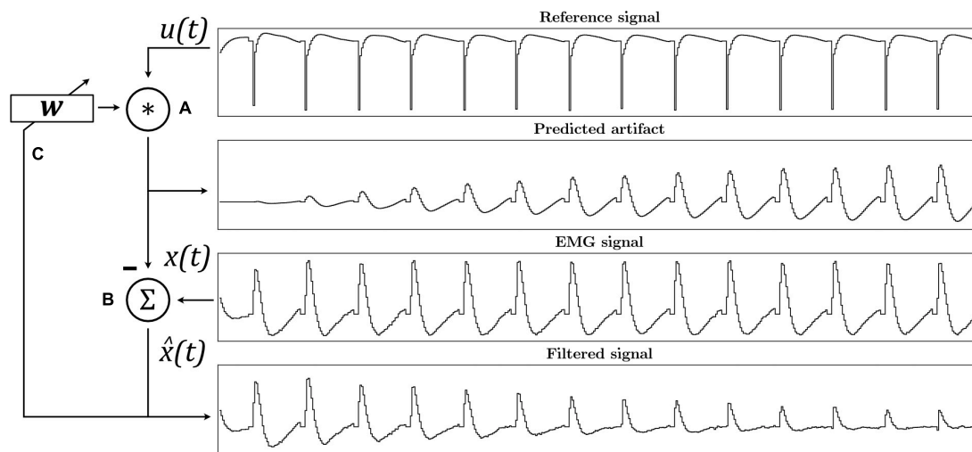
FIGURE 2 The \epsilon -Normalized Least Mean Squares ( \epsilon -NLMS) adaptive filter algorithm convolutes the reference signal u(t) with filter weights w to predict the artifact waveform (A). The predicted artifact is subtracted from the original signal x(t) to yield an estimated artifact-free signal \hat{x}(t) (B), which is then also used to update the filter weights after each sample (C).
