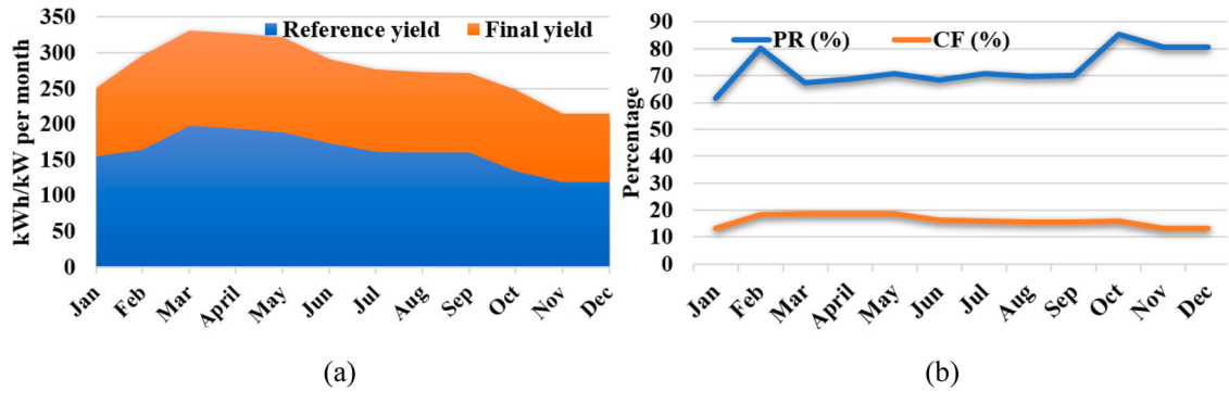
Figure 9. (a) System yield of the plant based on the actual performance and (b) actual PR and CF of the plant.
