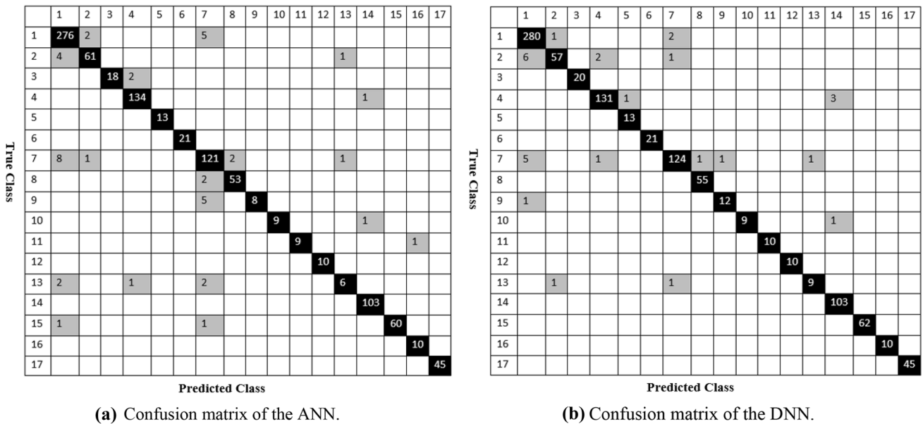
Fig. 5 Confusion matrices of the proposed tower graph and HLAP based ECG signal classification
