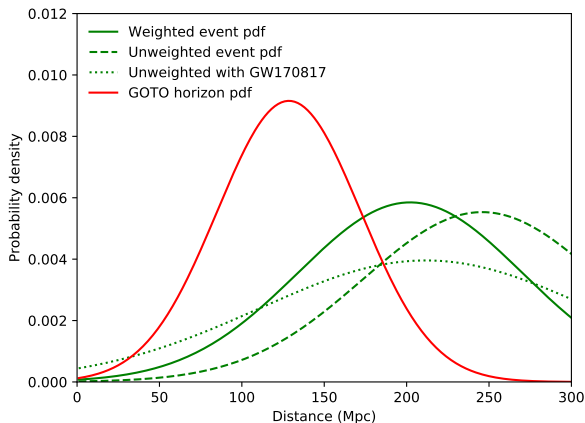
Figure 6. The probability density function (PDF) of the horizons achieved for a Bazin model during the 29 GOTO-4 LVC follow-up campaigns (red). These are compared to the weighted PDF (weights = 1/\sigma_{\text{dist}}^2 ) of the 5 BNS merger events during this time (green, solid), their unweighted PDF (dashed), and the unweighted PDF when the distance to GW170817 (41 Mpc; Hjorth et al. 2017) is included (dotted). The weighted PDF including GW170817 is not shown because the distance errors for this event are far smaller than the other 5 due to its EM detection.
