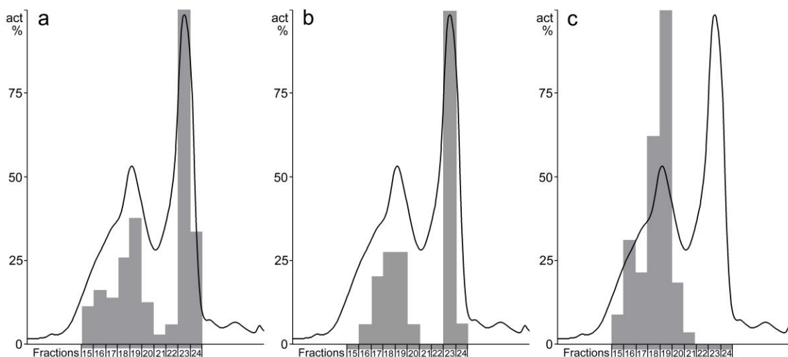
Figure 5. Distribution of the relative activities (a) N-acylation of methyl pipercolinate rac-5a , (b) hydrolysis of ethyl 3-butanamidobutanoate rac-1c and (c) hydrolysis of N-acetylmethionine rac-2a in the CAL-A Cat#ICR-112 gel filtration fractions. Activities shown as % in relation to the most active fraction.
