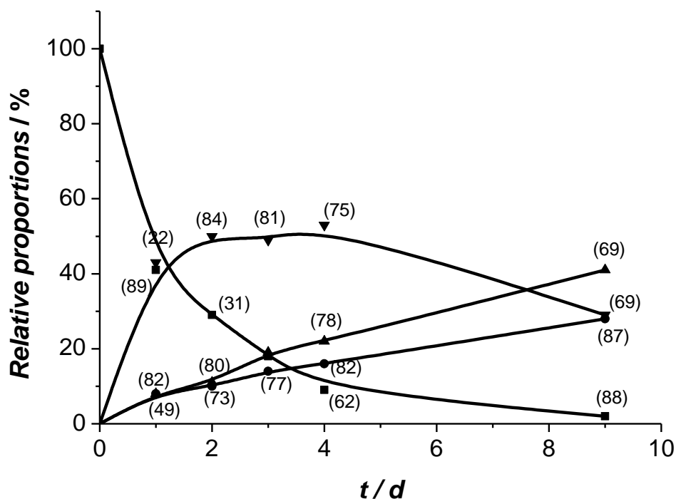
Figure 1. Cat#NZL-101-IMB-catalyzed ( 100 \text{ mg cm}^{-3} ) hydrolysis of rac - 1c (■, 0.050 M) and formation of the products ( S )- 1b (●), ( R )- 1a (▼) and ( R )- 1d (▲). Ee-values have been marked in parentheses.
