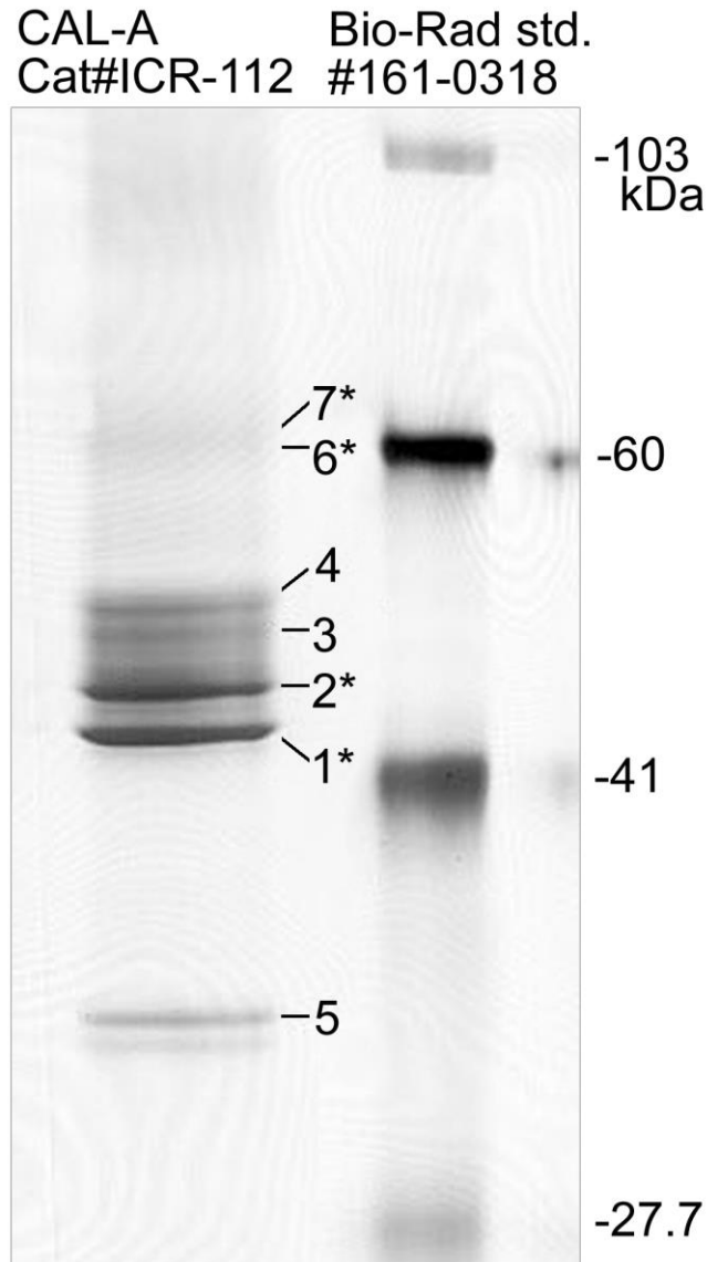
Figure 2. SDS-PAGE analysis (Bio-Rad Criterion 10% Bis-Tris/ silver stained) of the commercial CAL-A preparation (Cat#ICR-112 from Codexis) against Bio-Rad standard #161-0318. The bands submitted for in-gel digestion, LC-MS/MS analysis and sequence comparison are labeled 1-7. The best sequence hits: bands 1-2) CAL-A; bands 3-4) \alpha -amylase ( Aspergillus shirousami ); band 5) CAL-A N-terminal half; band 6) maltase glucoamylase ( Aspergillus ); band 7) maltase glucoamylase / serine carboxypeptidase ( Aspergillus ). Bands marked with * were only or additionally analyzed from fractionated samples.
