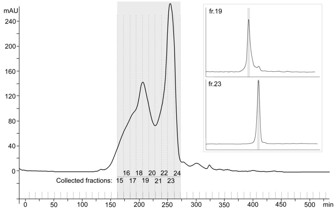
Figure 3. UV-Vis chromatogram of FPLC gel filtration fractionation of the CAL-A Cat#ICR-112. The fractions collected for analysis are highlighted. The smaller chromatograms show the peak fractions 19 and 23 after second round of gel filtration.
