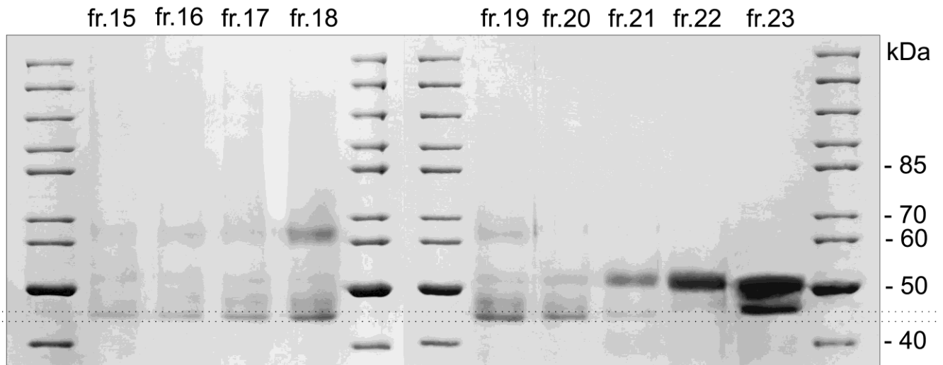
Figure 4. SDS-PAGE analysis of concentrated gel filtration fractions 15-23 of CAL-A Cat#ICR-112 against Fermentas Pageruler standard #SM0661 (self-casted 8% gel/ Coomassie Brilliant Blue stained). The two dotted horizontal lines between 40 kDa and 50 kDa show the migration fronts of the two CAL-A proteins. The collected fraction 24 is missing from the image.
