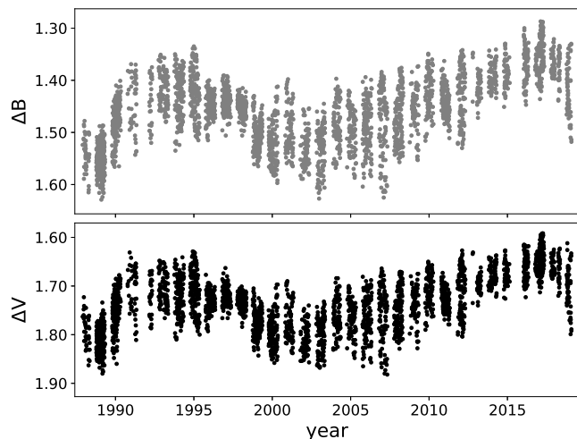
Fig. 1. Johnson B- and V-band differential photometry of LQ Hya.
