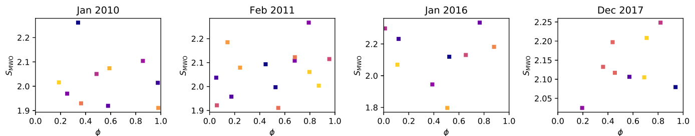
Fig. 4. Ca II H&K activity index S_{MWO} of LQ Hya as a function of rotation phase \phi . The four panels present the S_{MWO} values in each of the observing epochs, and the marker colours represent normalised time from the first (blue) to the last (yellow) observation within each observing run.
