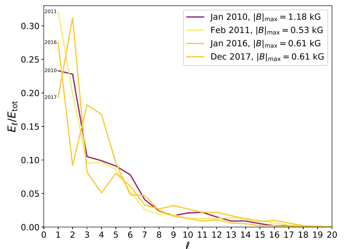
Fig. 7. Magnetic energy spectra of the ZDI maps as a function of the angular order \ell , normalised by the total magnetic energy E_{\text{tot}} . The line colours indicate the maximum field strength |B|_{\max} in each map, as given in the legend, darker colours denoting stronger fields.
