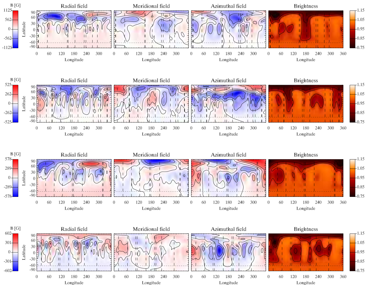
Fig. 6. Top to bottom: ZDI maps of LQ Hya in equirectangular projection from the epochs January 2010, February 2011, January 2016, and December 2017. In each epoch separate maps are shown for the radial, meridional, and azimuthal magnetic field components as well as the surface brightness distribution. The vertical lines in the maps denote the rotational phases of the individual observation and the horizontal line the lower limit of visibility due to the stellar inclination.
