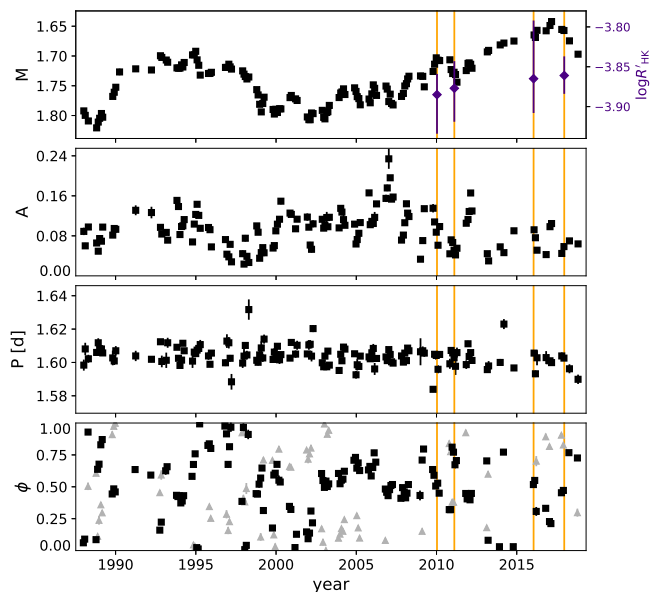
Fig. 5. Light curve mean magnitude M , amplitude A , period P , and phases of the light curve minima \phi_{\min} for LQ Hya. Both M and A are in the scale of \Delta V . The minimum phases are shown as black squares for the primary light curve minima and grey triangles for the secondary minima. The vertical orange lines denote the epochs of the ZDI maps. The average chromospheric activity levels \log R'_{HK} , corresponding to the ZDI maps, are shown in the top panel as violet diamonds with error bars indicating the variability ranges over the stellar rotation.
