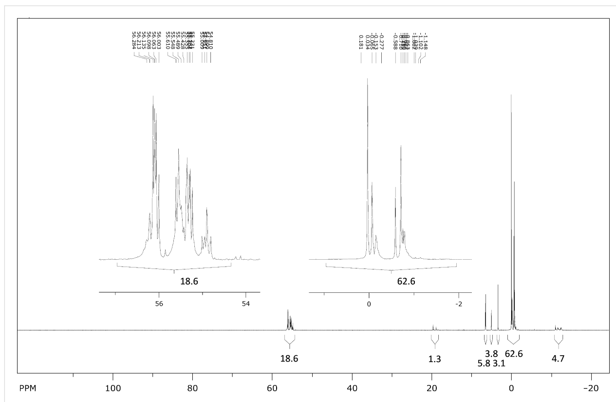
Figure 1: ^{31}\text{P} NMR spectrum (162 MHz, \text{D}_2\text{O} ) of the crude product mixture after refluxing equimolar amounts of thymidine and triethylammonium phosphite and 4 equiv of \text{S}_8 in toluene for 90 h.
