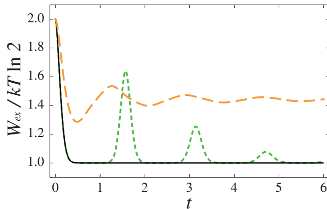
Figure 3. Time evolution of the extractable work of one qubit for an Ising model in a transverse field. We compared the dynamics for N = 4000 spins and three values of renormalized transverse field \lambda : \lambda^* = 1 (black solid line), \lambda^* = 0.1 (green short-dashed line) and \lambda^* = 1.9 (orange long-dashed line). The plots show how non-Markovian memory effects allow to retain or regain extractable work, leading to a thermodynamic enhancement compared to the Markovian case (black solid line).
