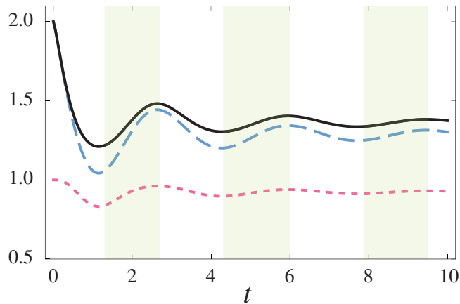
Figure 4. Time evolution of the extractable work (solid black line), the mutual information (blue long-dashed line) and system entropy (red short-dashed line), for the amplitude damping photonics band gap model, with detuning from the band gap edge frequency \delta = -1 (a.u.). The green shaded regions highlight time intervals in which one observes a partial recovery of the extractable work even though the system entropy increases.
