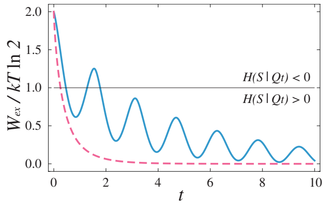
Figure 2. Time evolution of the extractable work W_{ex}/kT \ln 2 for one qubit system. The blue solid line corresponds to a Pauli channel model with decay rates \gamma_1(t) = \gamma_2(t) = \lambda/2 , and \gamma_3(t) = \omega \tan(\omega t)/2 , with \lambda = 0.1 and \omega = 2 (a.u.). The red dashed line corresponds to a Pauli channel model 37 with decay rates \gamma_1(t) = \gamma_2(t) = \lambda/2 , and \gamma_3(t) = -\omega \tanh(\omega t)/2 , with \lambda = 1 and \omega = 0.5 (a.u.). In both cases the dynamical map is non-divisible but only in one scenario (blue solid line) revivals of work extraction are present.
