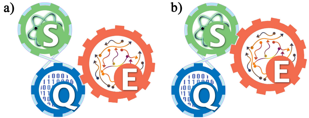
Figure 1. Illustration of the two physical scenarios considered in the Article. We consider a system S given access to a quantum memory Q under natural conditions: in (a), the memory Q is subject to interaction with an environment E (open quantum memory); in (b) it is the system S that is coupled with the environment (open quantum system).
